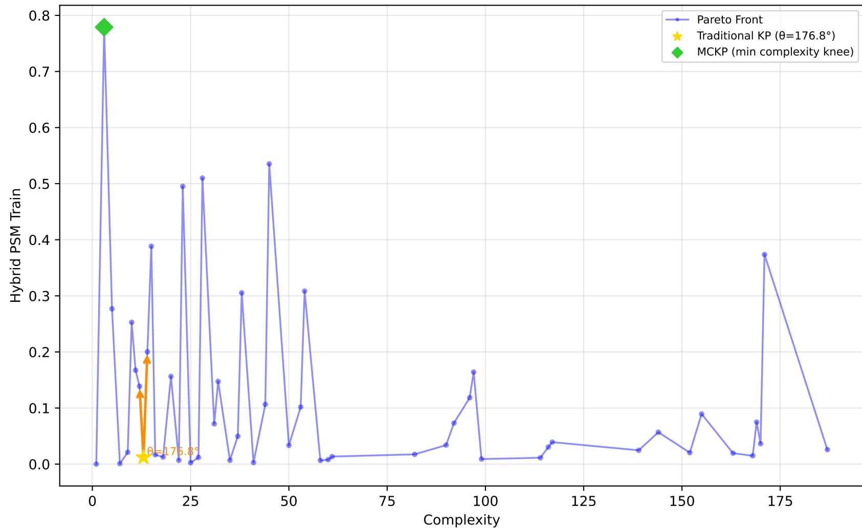
678_visualizing_environmental - Run 21 - MVP - Hybrid PSM Train \lambda_1=0.00, \lambda_2=0.00, \lambda_3=0.10 | Difficulty: 0.09 | Method: mckp
