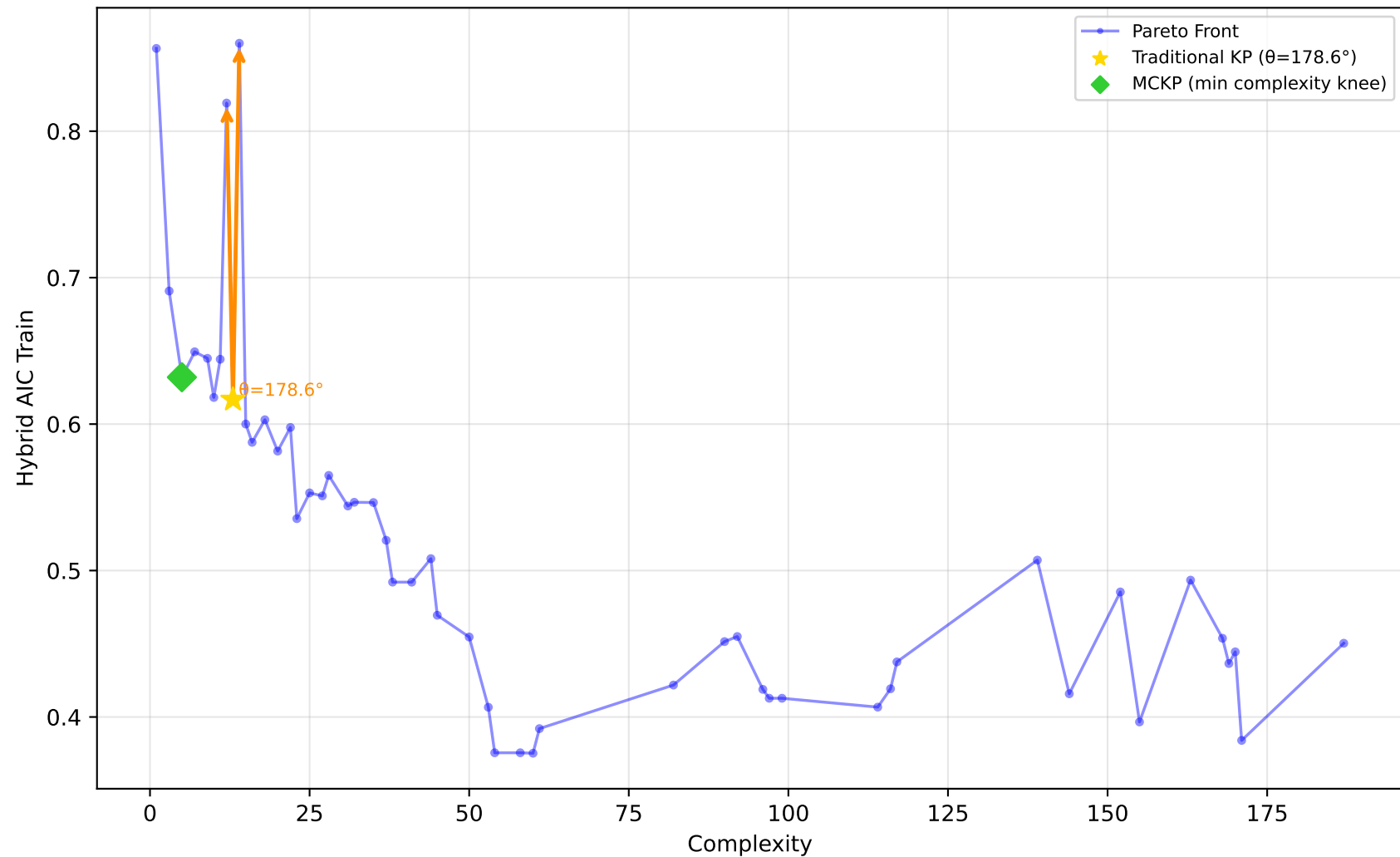
678_visualizing_environmental - Run 21 - SVP - Hybrid AIC Train \lambda_1=0.00, \lambda_2=0.10, \lambda_3=0.20 | Difficulty: 0.09 | Method: mckp
