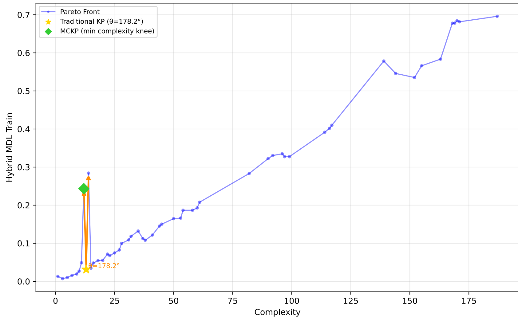
678_visualizing_environmental - Run 21 - SVP - Hybrid MDL Train \lambda_1=0.00, \lambda_2=0.10, \lambda_3=0.20 | Difficulty: 0.09 | Method: mckp
