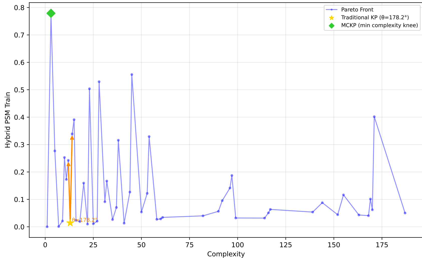
678_visualizing_environmental - Run 21 - SVP - Hybrid PSM Train \lambda_1=0.00, \lambda_2=0.10, \lambda_3=0.20 | Difficulty: 0.09 | Method: mckp
