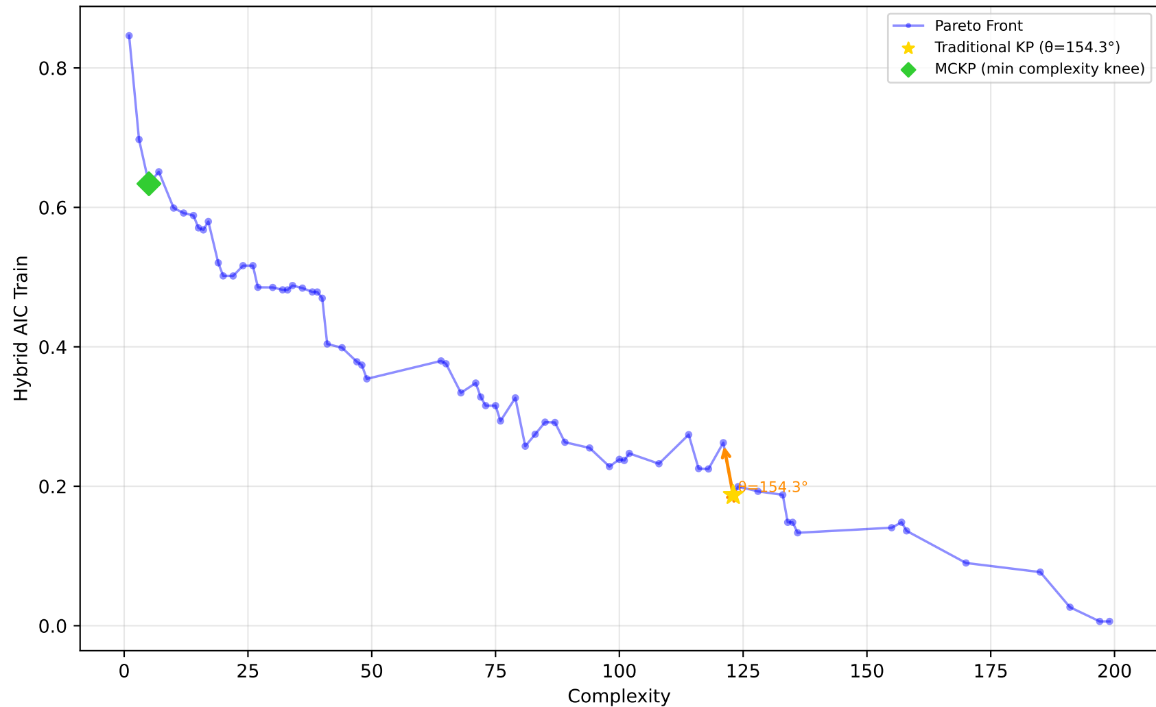
678_visualizing_environmental - Run 22 - MVP - Hybrid AIC Train \lambda_1=0.00, \lambda_2=0.00, \lambda_3=0.10 | Difficulty: 0.31 | Method: mckp
