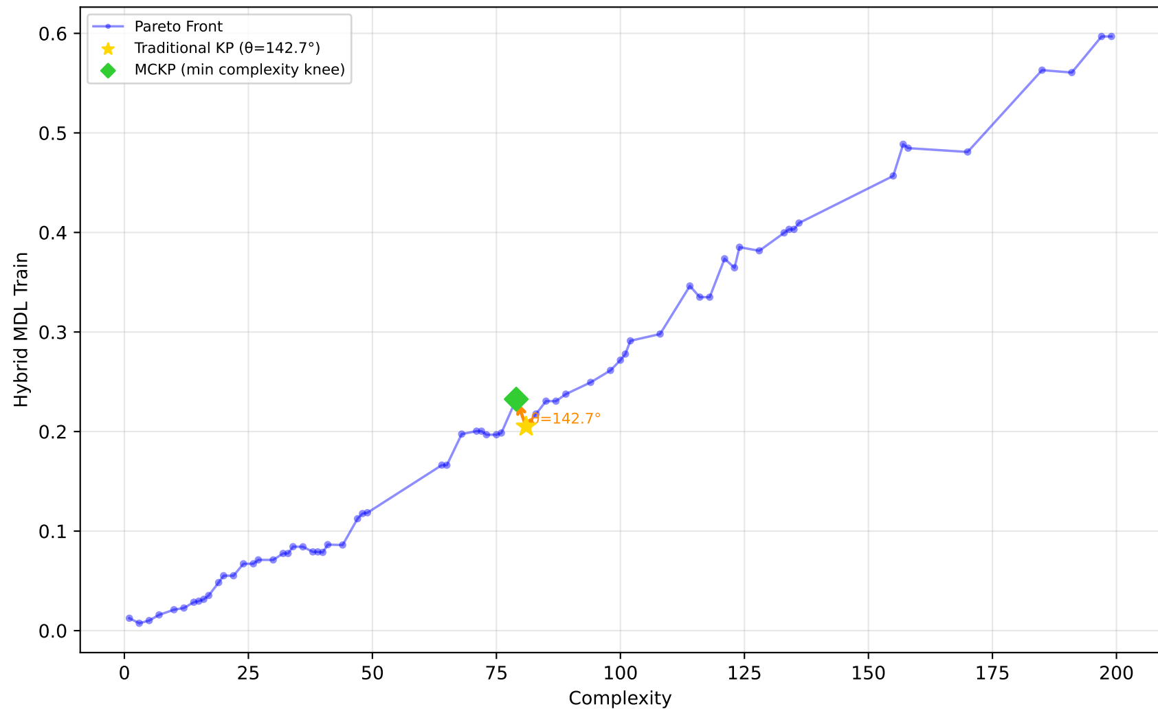
678_visualizing_environmental - Run 22 - MVP - Hybrid MDL Train \lambda_1=0.00, \lambda_2=0.00, \lambda_3=0.10 | Difficulty: 0.31 | Method: mckp
