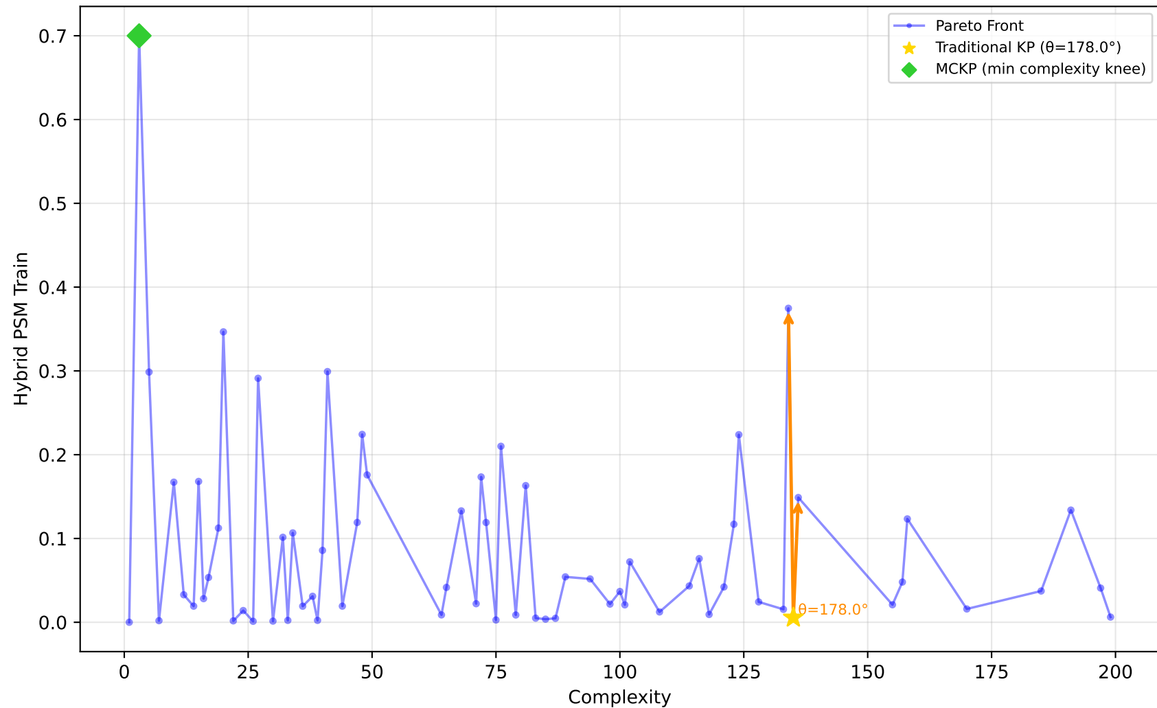
678_visualizing_environmental - Run 22 - MVP - Hybrid PSM Train \lambda_1=0.00, \lambda_2=0.00, \lambda_3=0.10 | Difficulty: 0.31 | Method: mckp
