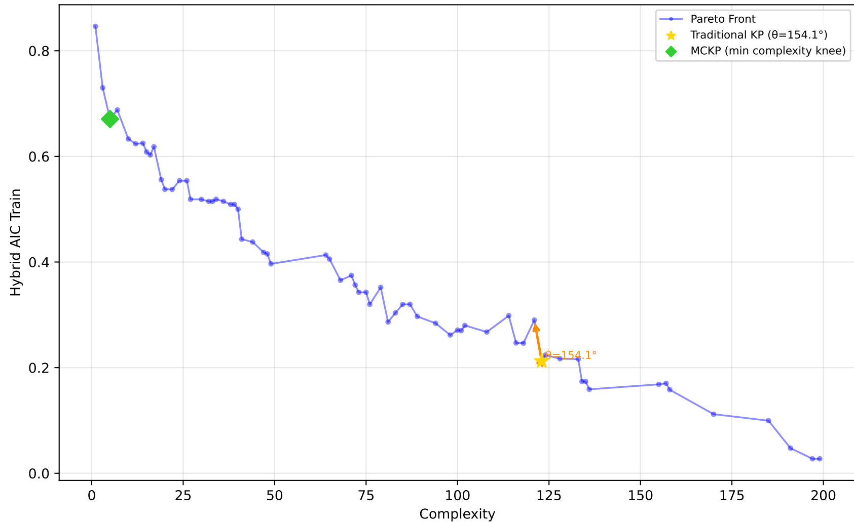
678_visualizing_environmental - Run 22 - SVP - Hybrid AIC Train \lambda_1=0.40, \lambda_2=0.00, \lambda_3=0.00 | Difficulty: 0.31 | Method: mckp
