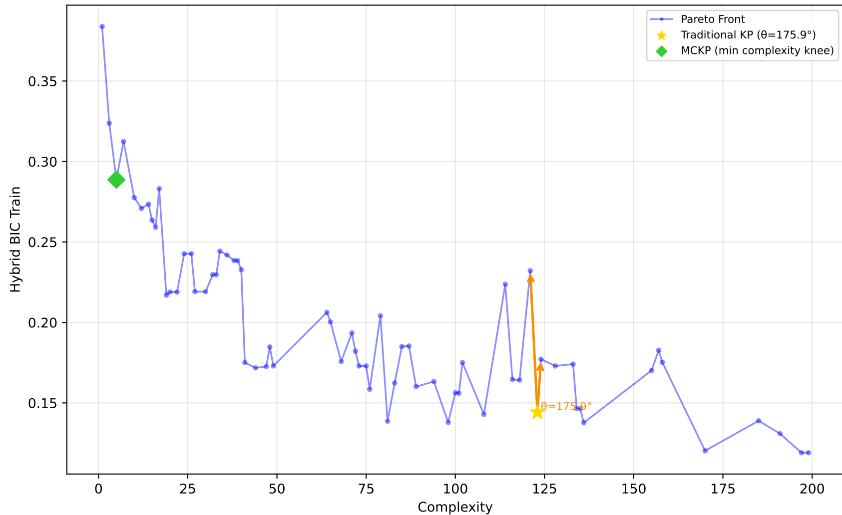
678_visualizing_environmental - Run 22 - SVP - Hybrid BIC Train \lambda_1=0.40, \lambda_2=0.00, \lambda_3=0.00 | Difficulty: 0.31 | Method: mckp
