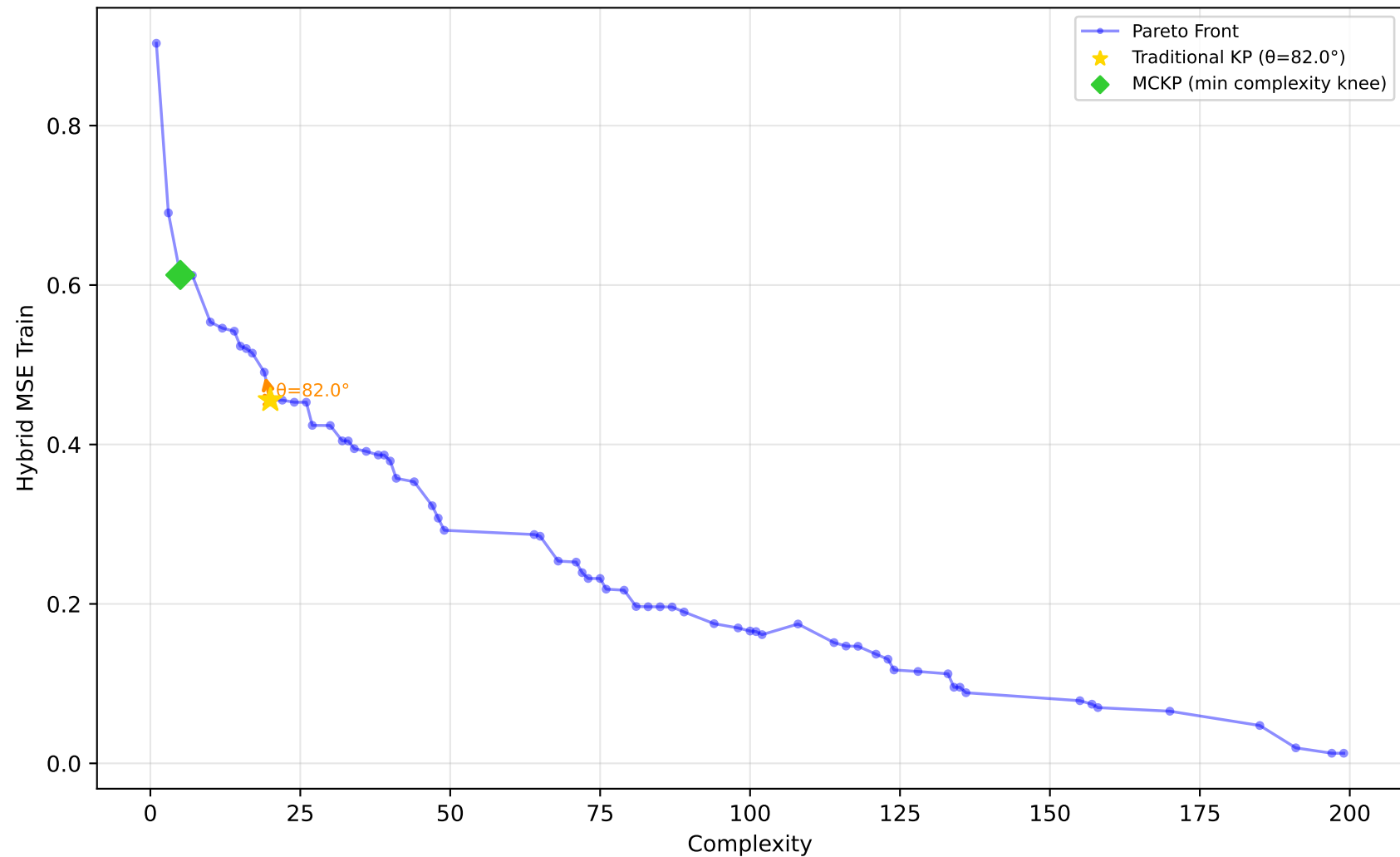
678_visualizing_environmental - Run 22 - SVP - Hybrid MSE Train \lambda_1=0.00, \lambda_2=0.10, \lambda_3=0.20 | Difficulty: 0.31 | Method: mckp
