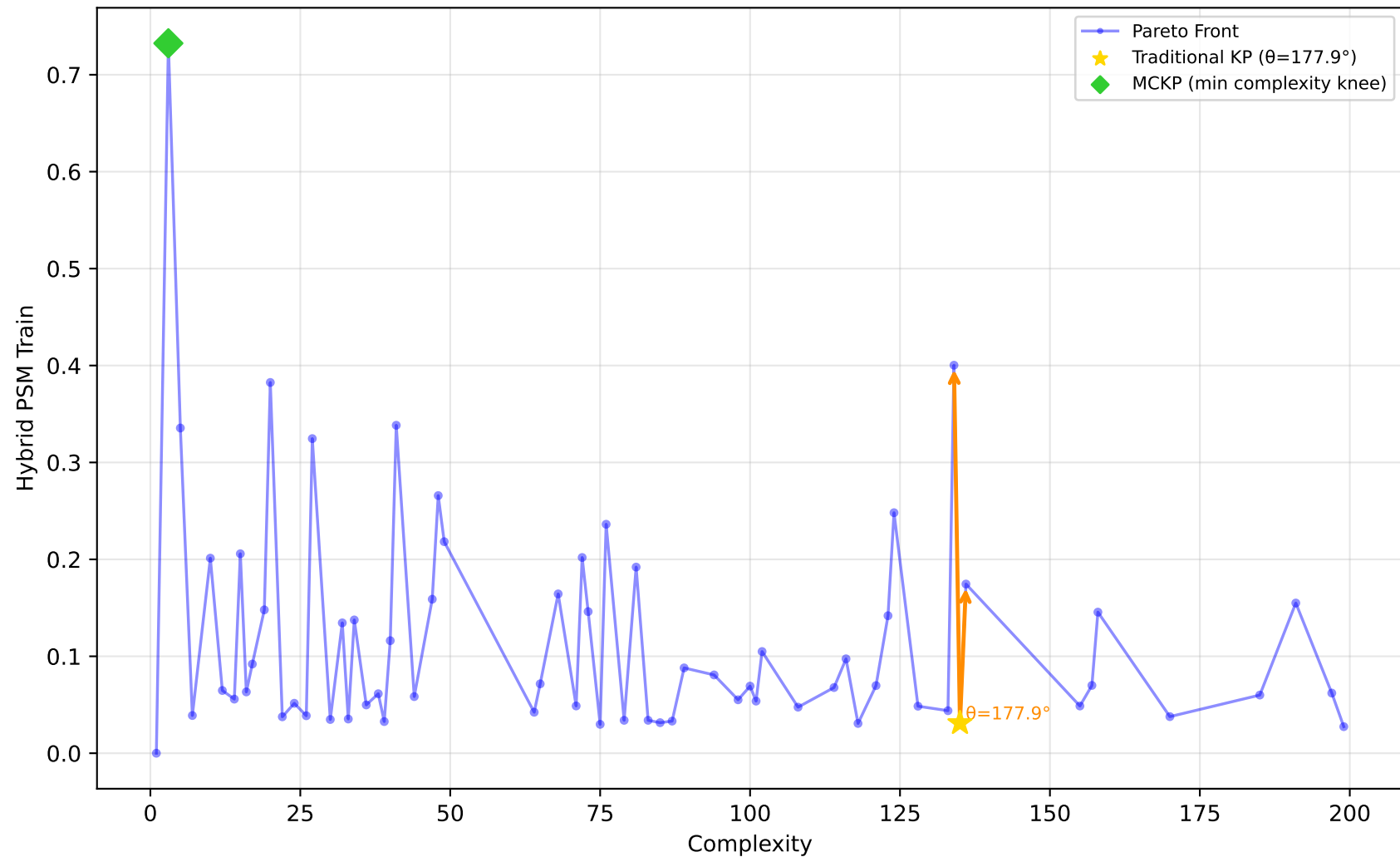
678_visualizing_environmental - Run 22 - SVP - Hybrid PSM Train \lambda_1=0.40, \lambda_2=0.00, \lambda_3=0.00 | Difficulty: 0.31 | Method: mckp
