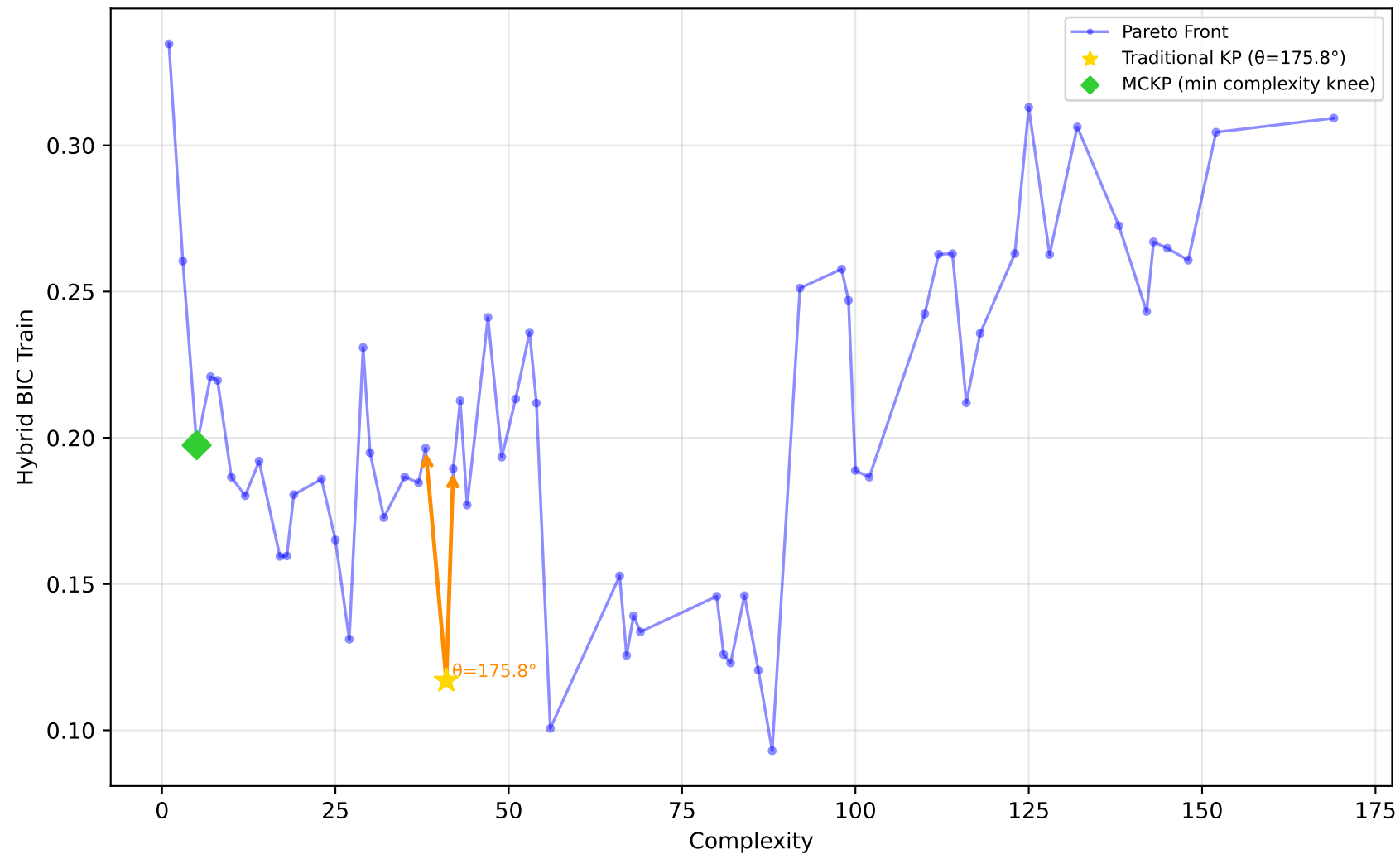
678_visualizing_environmental - Run 24 - MVP - Hybrid BIC Train \lambda_1=0.40, \lambda_2=0.00, \lambda_3=0.00 | Difficulty: 0.08 | Method: mckp
