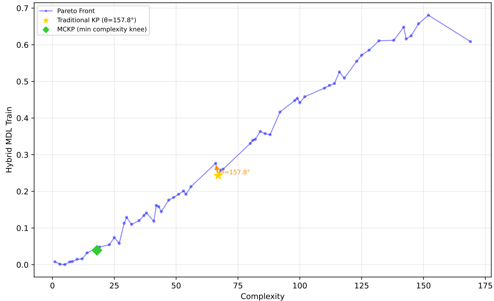
678_visualizing_environmental - Run 24 - MVP - Hybrid MDL Train \lambda_1=0.00 , \lambda_2=0.00 , \lambda_3=0.10 | Difficulty: 0.08 | Method: mckp
