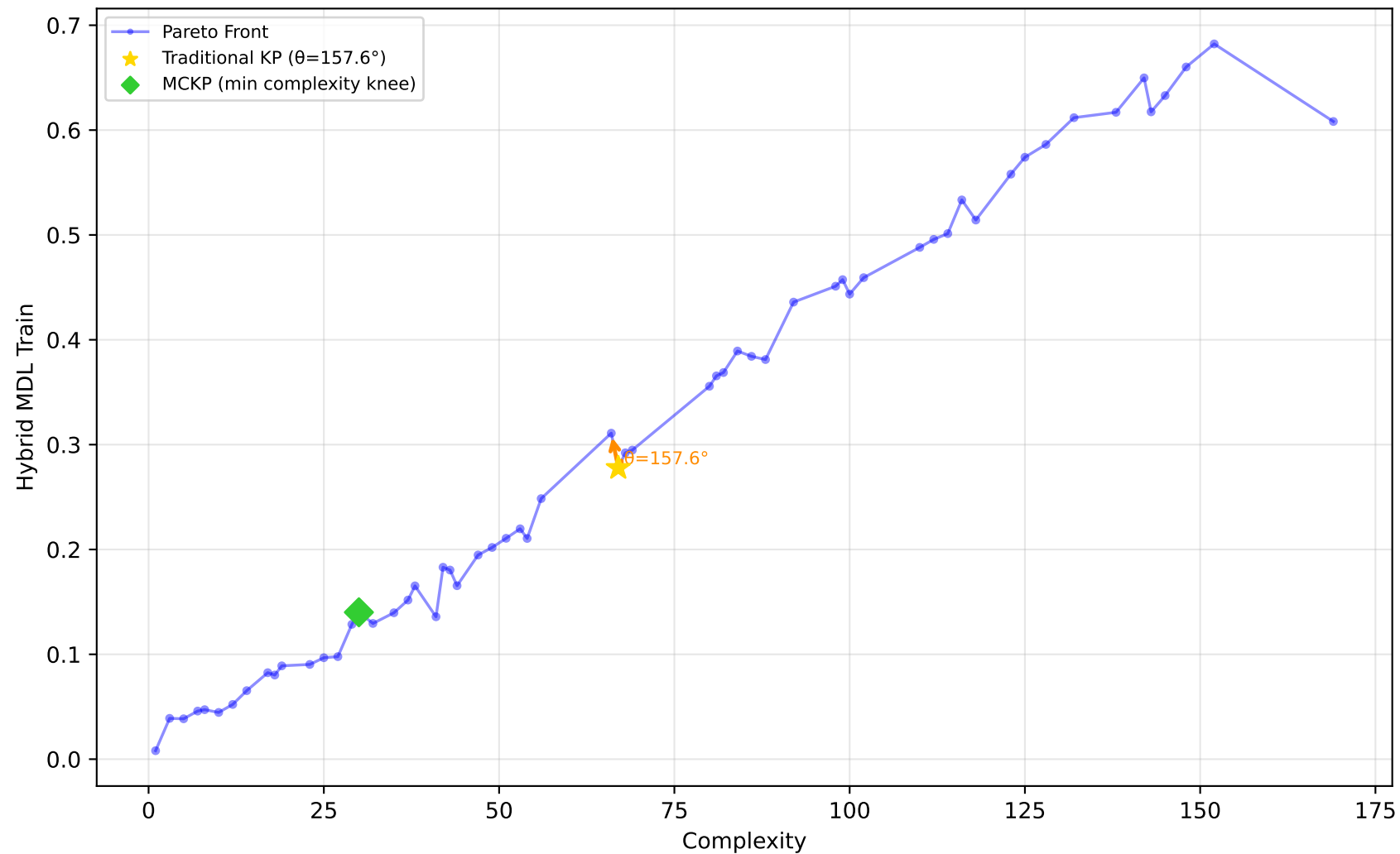
678_visualizing_environmental - Run 24 - MVP - Hybrid MDL Train \lambda_1=0.40 , \lambda_2=0.00 , \lambda_3=0.00 | Difficulty: 0.08 | Method: mckp
