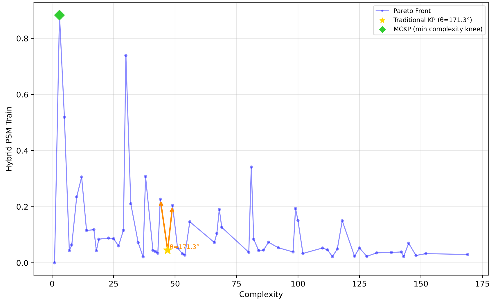
678_visualizing_environmental - Run 24 - MVP - Hybrid PSM Train \lambda_1=0.40 , \lambda_2=0.00 , \lambda_3=0.00 | Difficulty: 0.08 | Method: mckp
