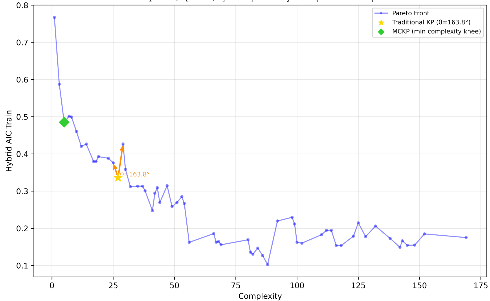
678_visualizing_environmental - Run 24 - SVP - Hybrid AIC Train \lambda_1=0.00 , \lambda_2=0.10 , \lambda_3=0.20 | Difficulty: 0.08 | Method: mckp
