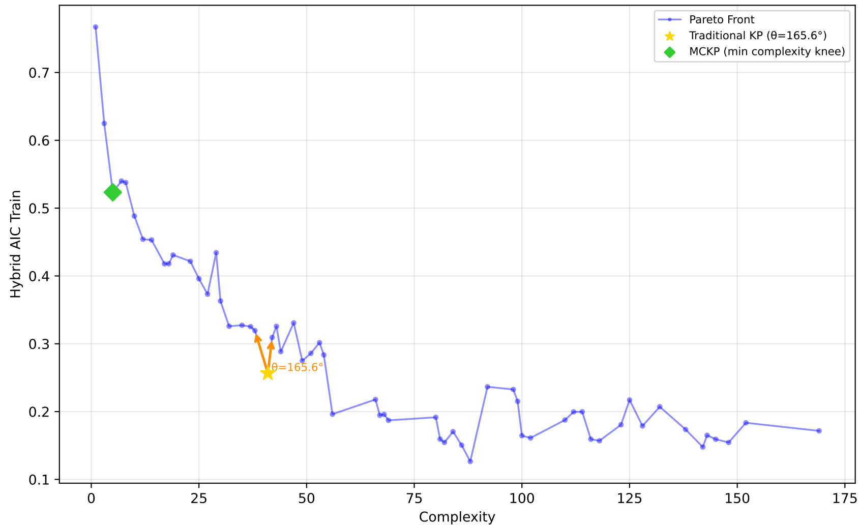
678_visualizing_environmental - Run 24 - SVP - Hybrid AIC Train \lambda_1=0.40 , \lambda_2=0.00 , \lambda_3=0.00 | Difficulty: 0.08 | Method: mckp
