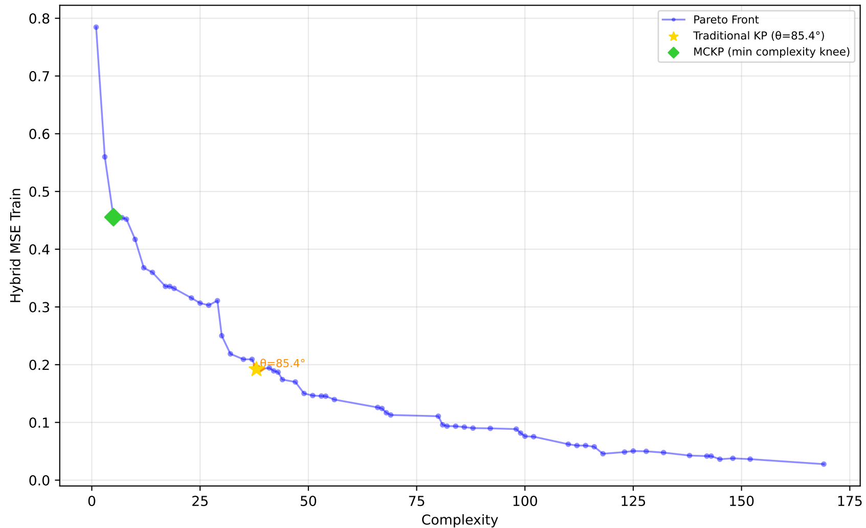
678_visualizing_environmental - Run 24 - SVP - Hybrid MSE Train \lambda_1=0.00, \lambda_2=0.10, \lambda_3=0.20 | Difficulty: 0.08 | Method: mckp
