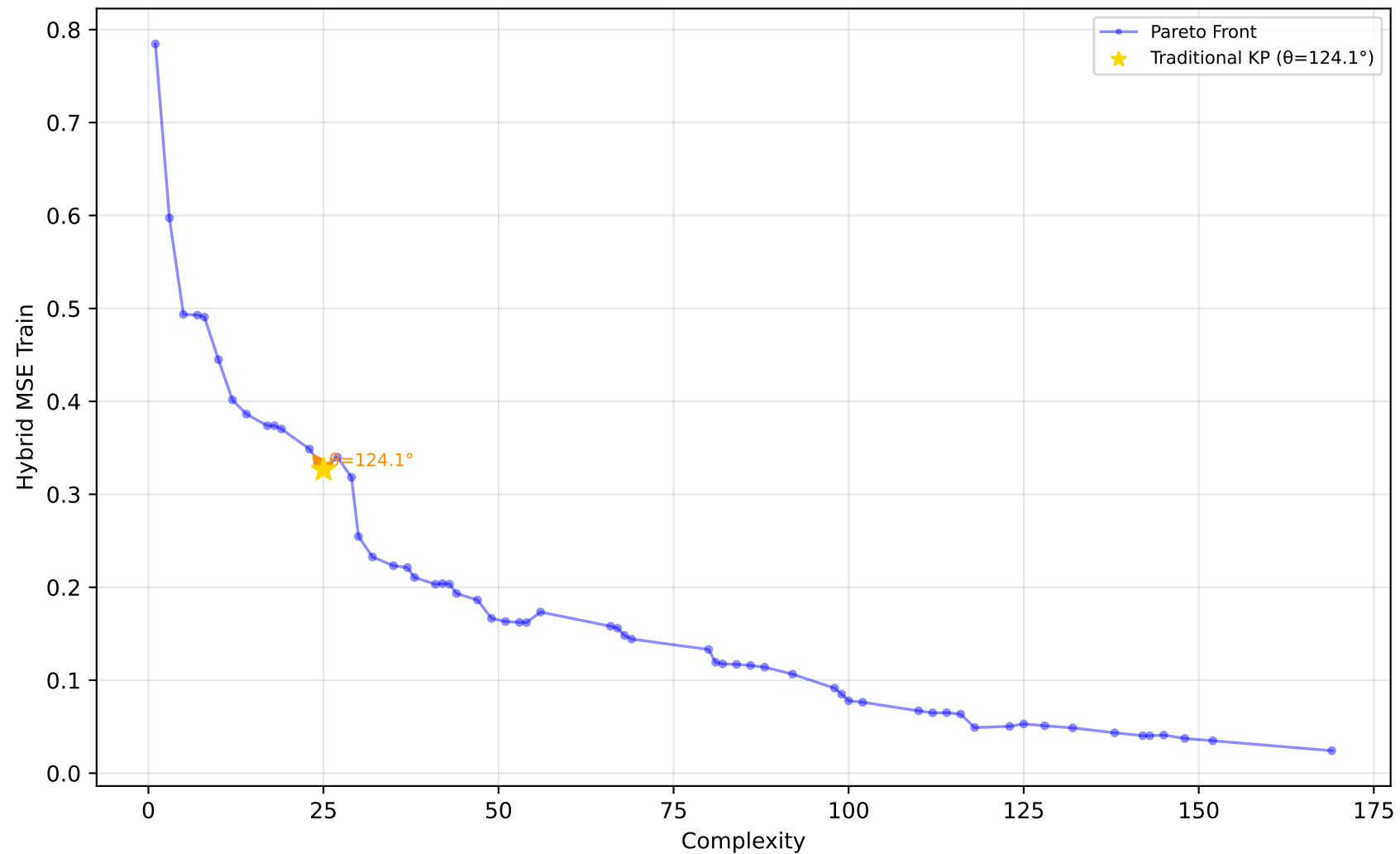
678_visualizing_environmental - Run 24 - SVP - Hybrid MSE Train \lambda_1=0.40 , \lambda_2=0.00 , \lambda_3=0.00 | Difficulty: 0.08 | Method: mckp
