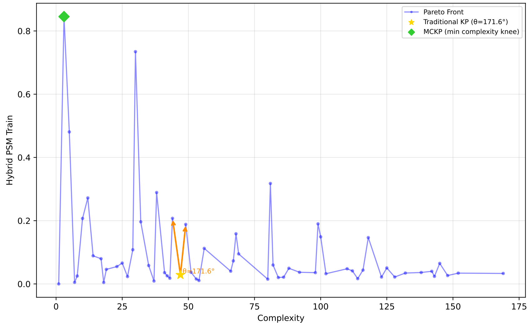
678_visualizing_environmental - Run 24 - SVP - Hybrid PSM Train \lambda_1=0.00 , \lambda_2=0.10 , \lambda_3=0.20 | Difficulty: 0.08 | Method: mckp
