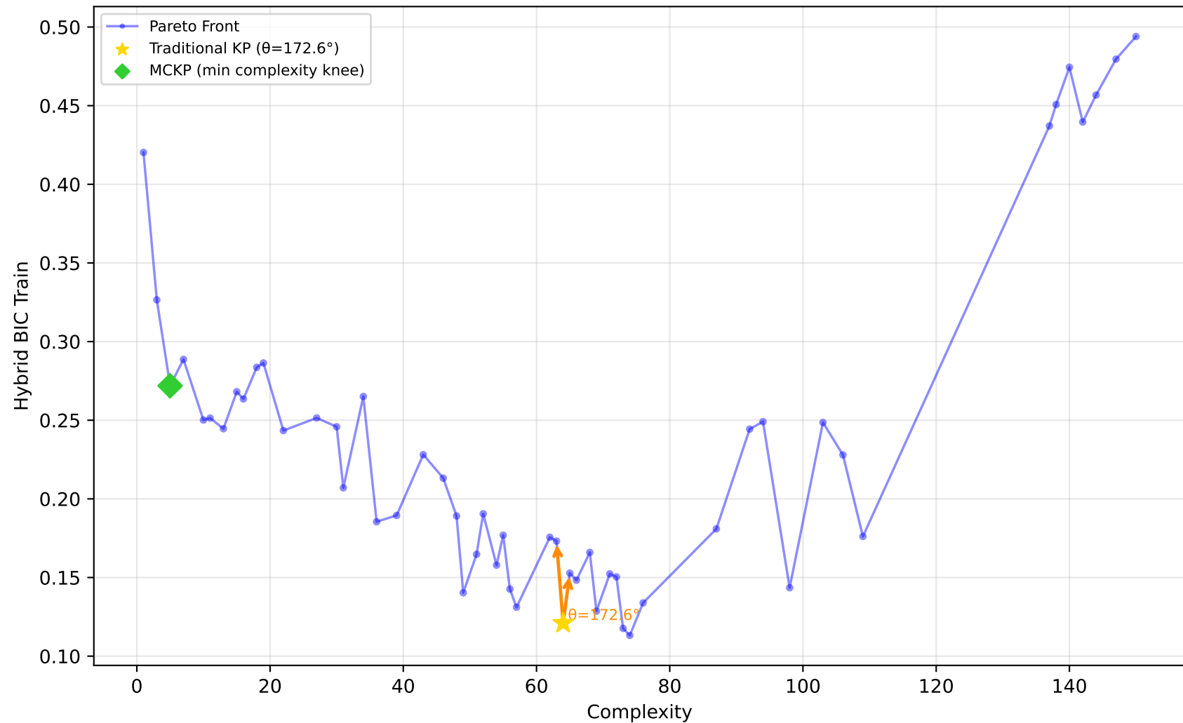
678_visualizing_environmental - Run 25 - MVP - Hybrid BIC Train \lambda_1=0.40, \lambda_2=0.00, \lambda_3=0.00 | Difficulty: 0.14 | Method: mckp
