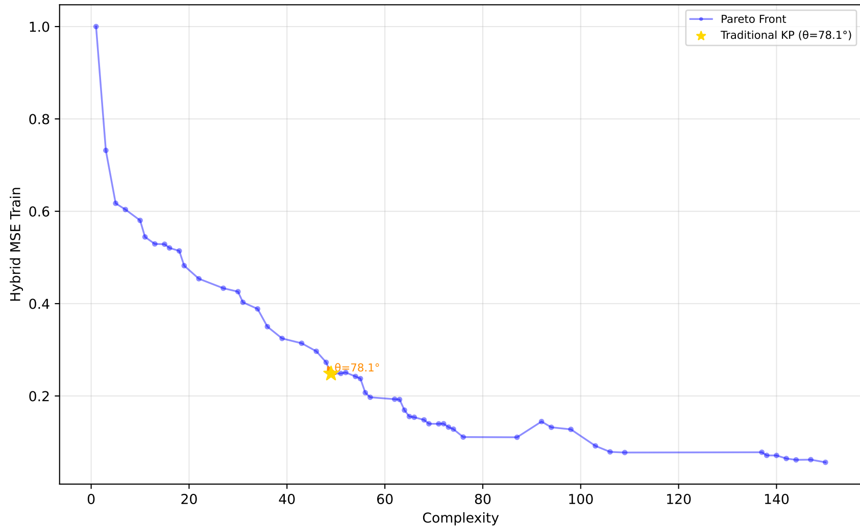
678_visualizing_environmental - Run 25 - MVP - Hybrid MSE Train \lambda_1=0.40 , \lambda_2=0.00 , \lambda_3=0.00 | Difficulty: 0.14 | Method: mckp
