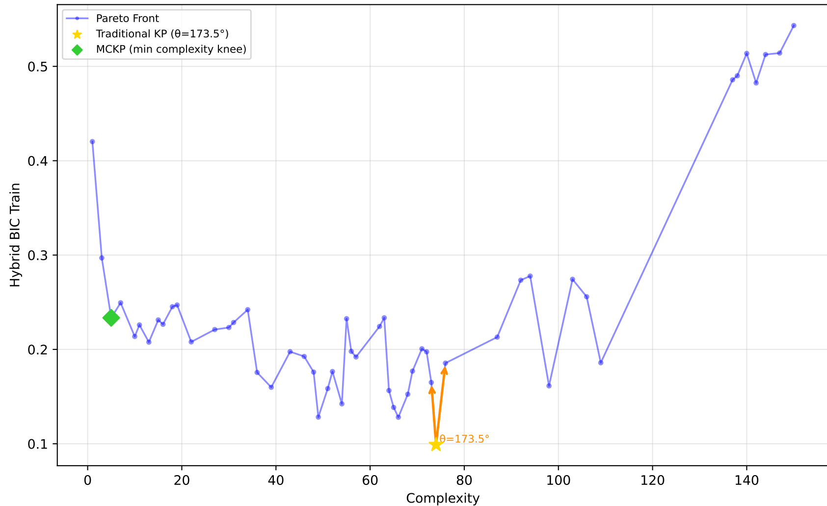
678_visualizing_environmental - Run 25 - SVP - Hybrid BIC Train \lambda_1=0.00, \lambda_2=0.10, \lambda_3=0.20 | Difficulty: 0.14 | Method: mckp
