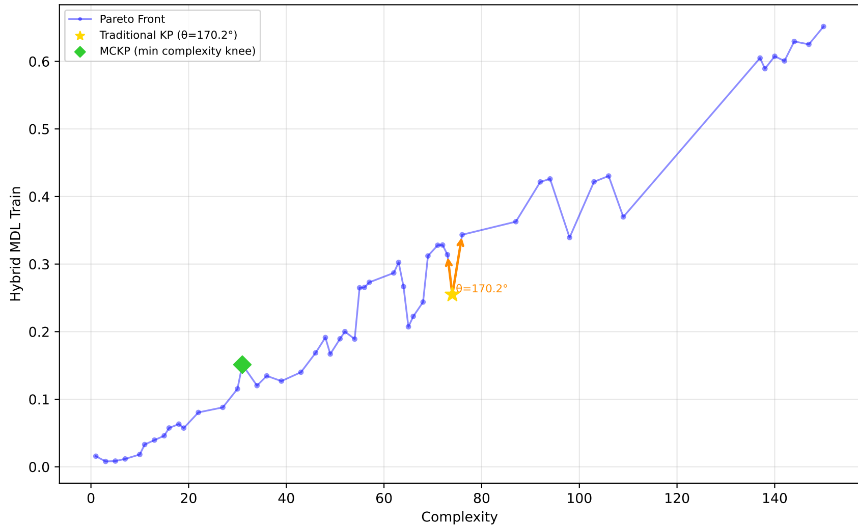
678_visualizing_environmental - Run 25 - SVP - Hybrid MDL Train \lambda_1=0.00, \lambda_2=0.10, \lambda_3=0.20 | Difficulty: 0.14 | Method: mckp
