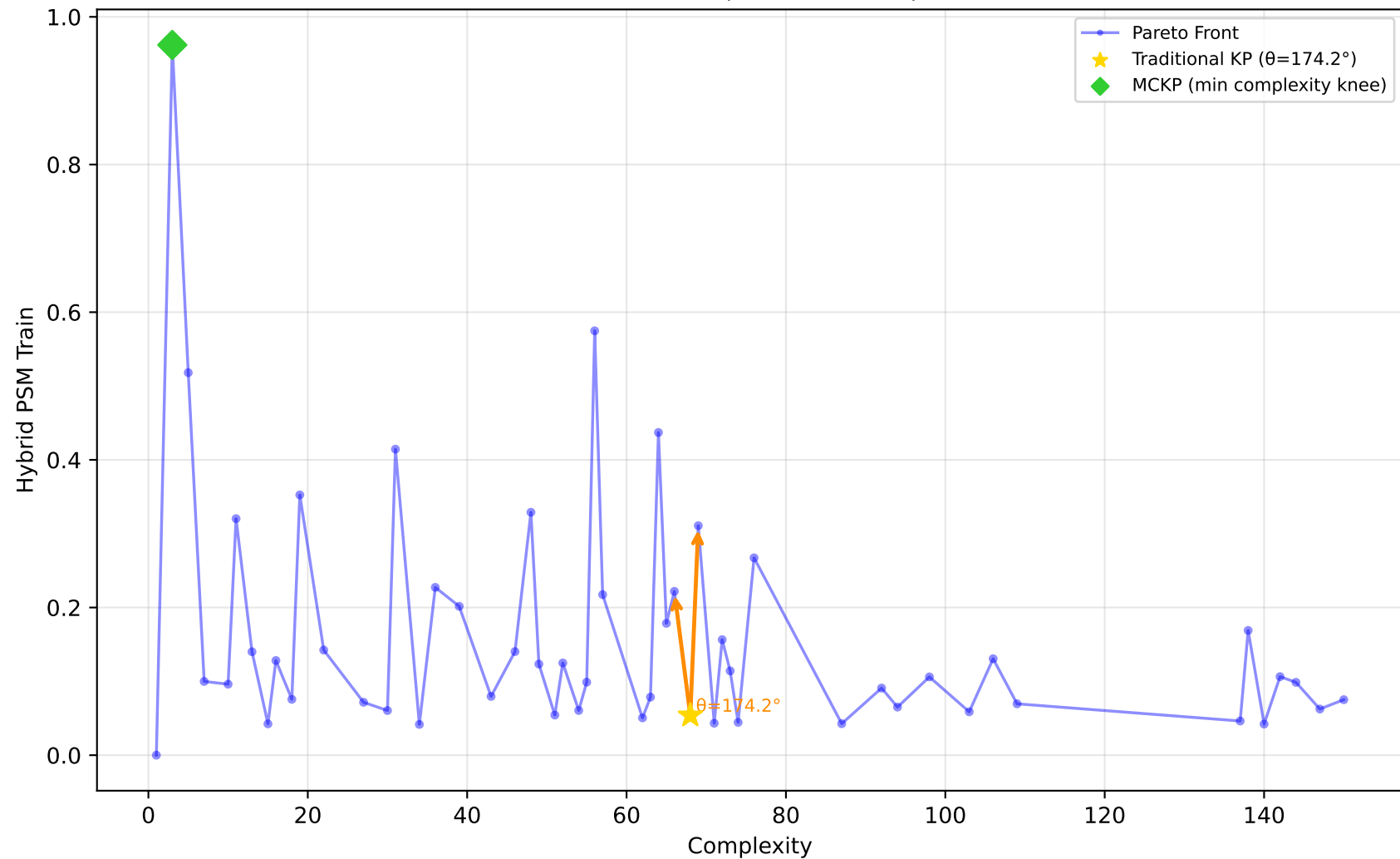
678_visualizing_environmental - Run 25 - SVP - Hybrid PSM Train \lambda_1=0.40, \lambda_2=0.00, \lambda_3=0.00 | Difficulty: 0.14 | Method: mckp
