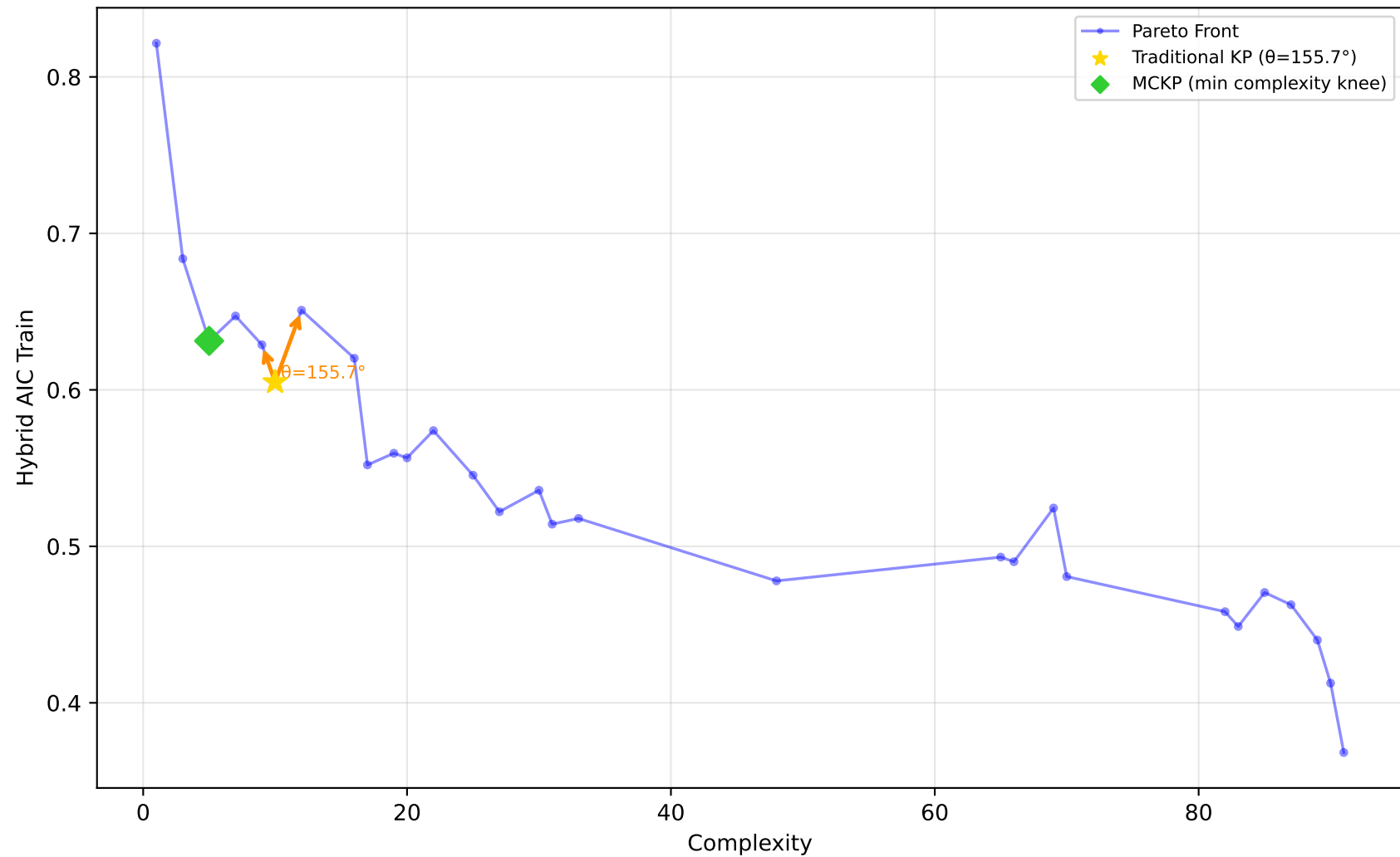
678_visualizing_environmental - Run 26 - MVP - Hybrid AIC Train \lambda_1=0.00, \lambda_2=0.00, \lambda_3=0.10 | Difficulty: 0.32 | Method: mckp
