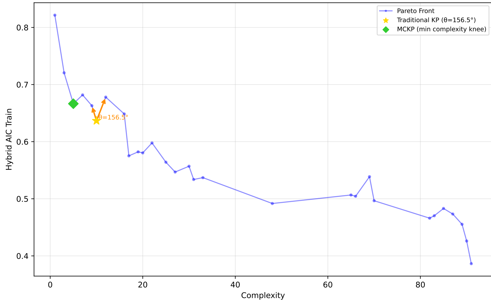
678_visualizing_environmental - Run 26 - MVP - Hybrid AIC Train \lambda_1=0.40 , \lambda_2=0.00 , \lambda_3=0.00 | Difficulty: 0.32 | Method: mckp
