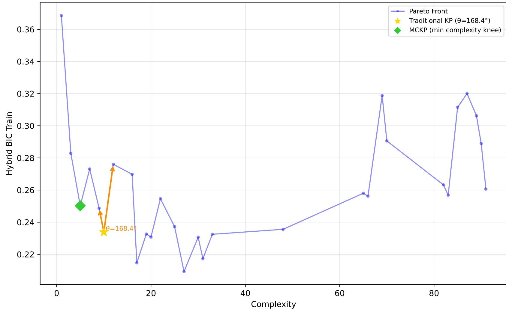
678_visualizing_environmental - Run 26 - MVP - Hybrid BIC Train \lambda_1=0.00, \lambda_2=0.00, \lambda_3=0.10 | Difficulty: 0.32 | Method: mckp
