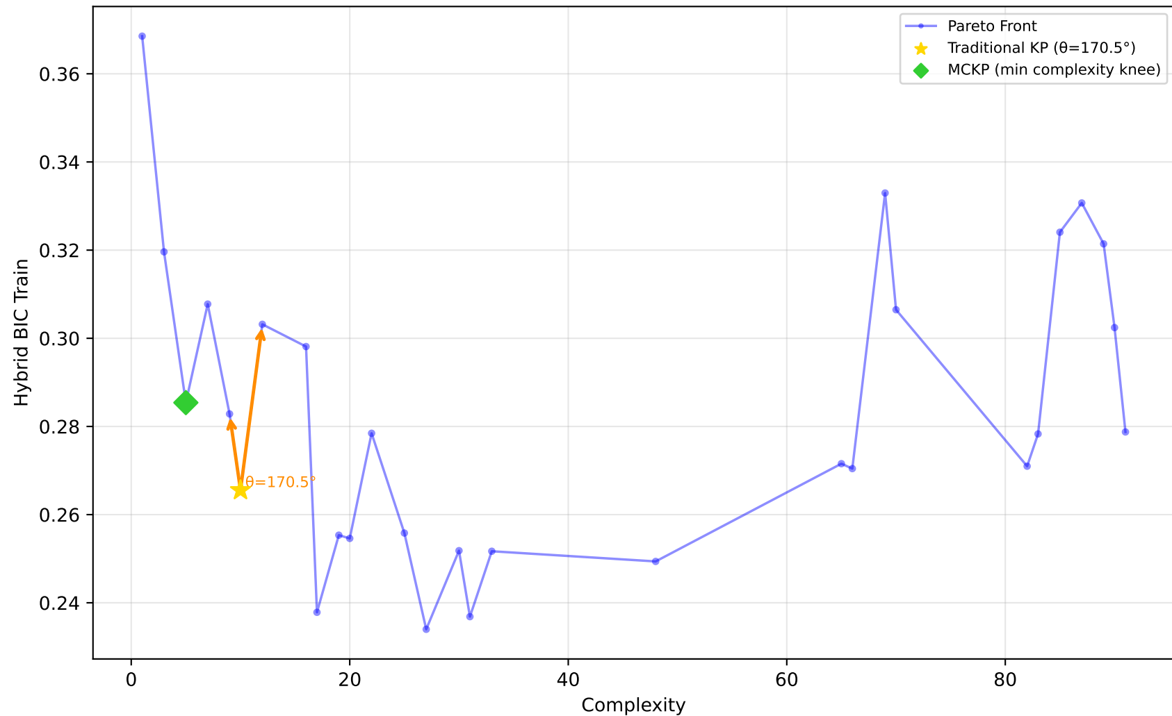
678_visualizing_environmental - Run 26 - MVP - Hybrid BIC Train \lambda_1=0.40, \lambda_2=0.00, \lambda_3=0.00 | Difficulty: 0.32 | Method: mckp
