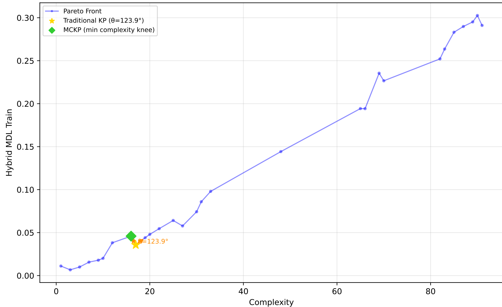
678_visualizing_environmental - Run 26 - MVP - Hybrid MDL Train \lambda_1=0.00, \lambda_2=0.00, \lambda_3=0.10 | Difficulty: 0.32 | Method: mckp
