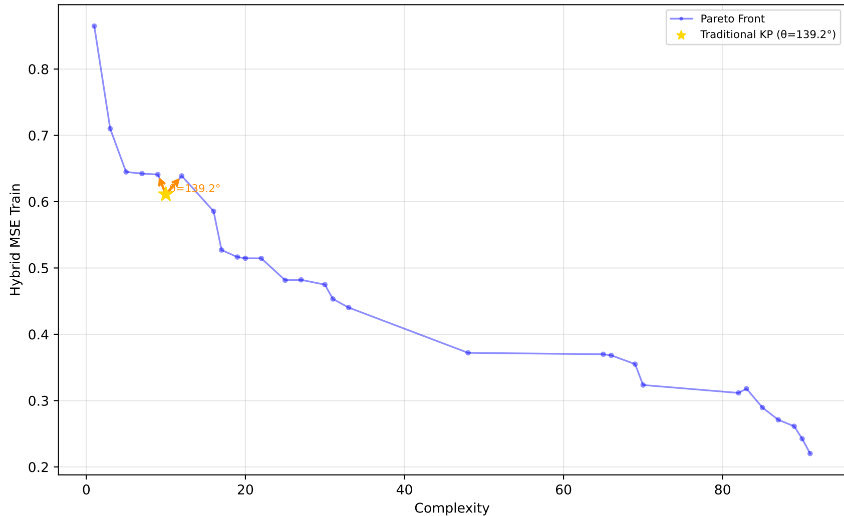
678_visualizing_environmental - Run 26 - SVP - Hybrid MSE Train \lambda_1=0.40 , \lambda_2=0.00 , \lambda_3=0.00 | Difficulty: 0.32 | Method: mckp
