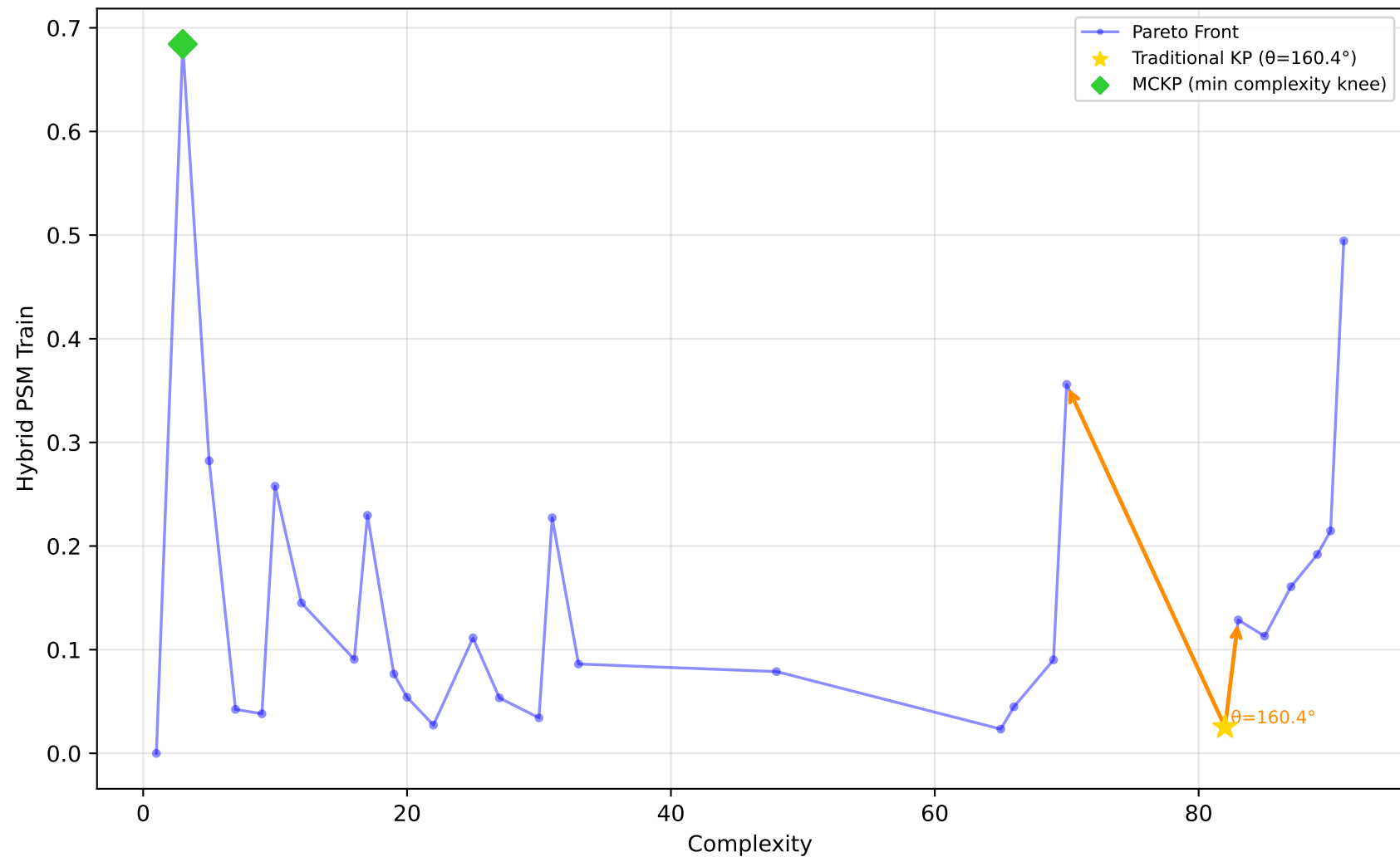
678_visualizing_environmental - Run 26 - SVP - Hybrid PSM Train \lambda_1=0.40 , \lambda_2=0.00 , \lambda_3=0.00 | Difficulty: 0.32 | Method: mckp
