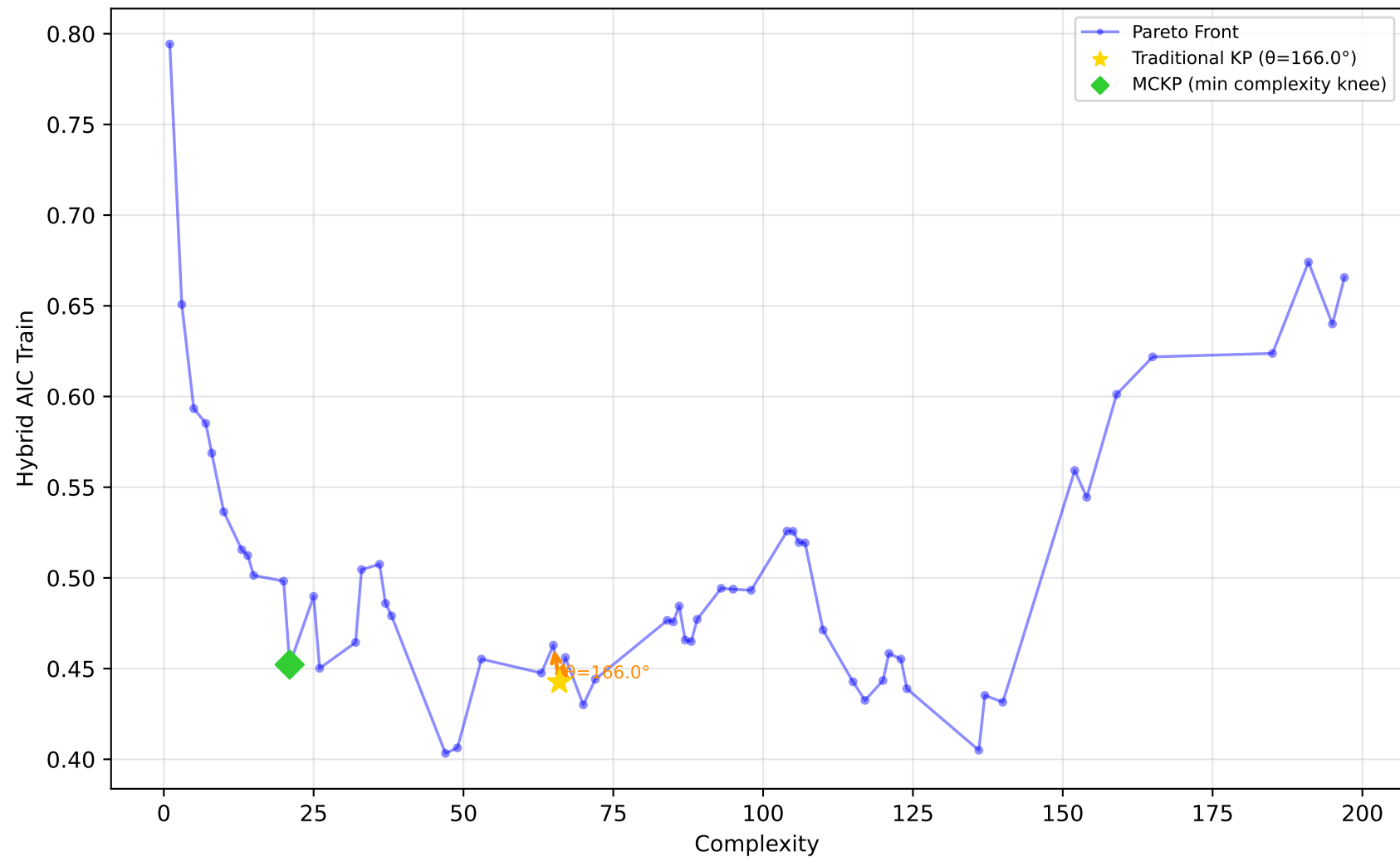
678_visualizing_environmental - Run 27 - MVP - Hybrid AIC Train \lambda_1=0.00, \lambda_2=0.00, \lambda_3=0.10 | Difficulty: 0.80 | Method: hmr
