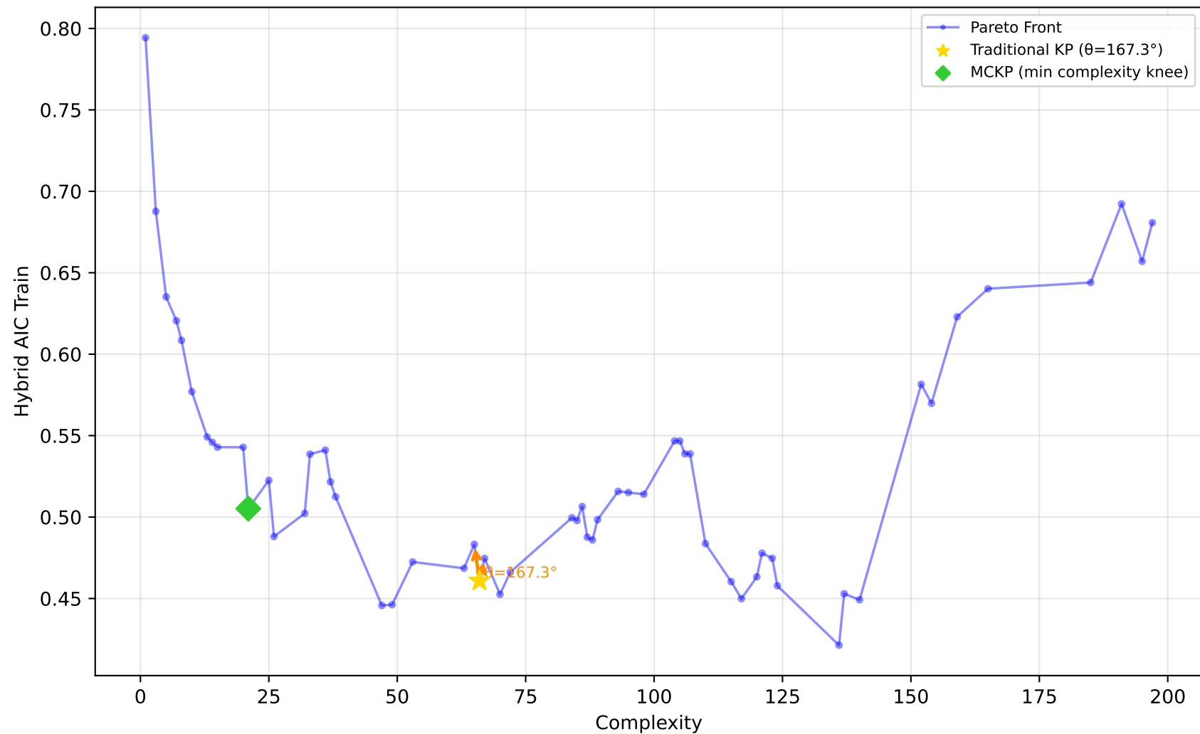
678_visualizing_environmental - Run 27 - SVP - Hybrid AIC Train \lambda_1=0.40, \lambda_2=0.00, \lambda_3=0.00 | Difficulty: 0.80 | Method: hmr
