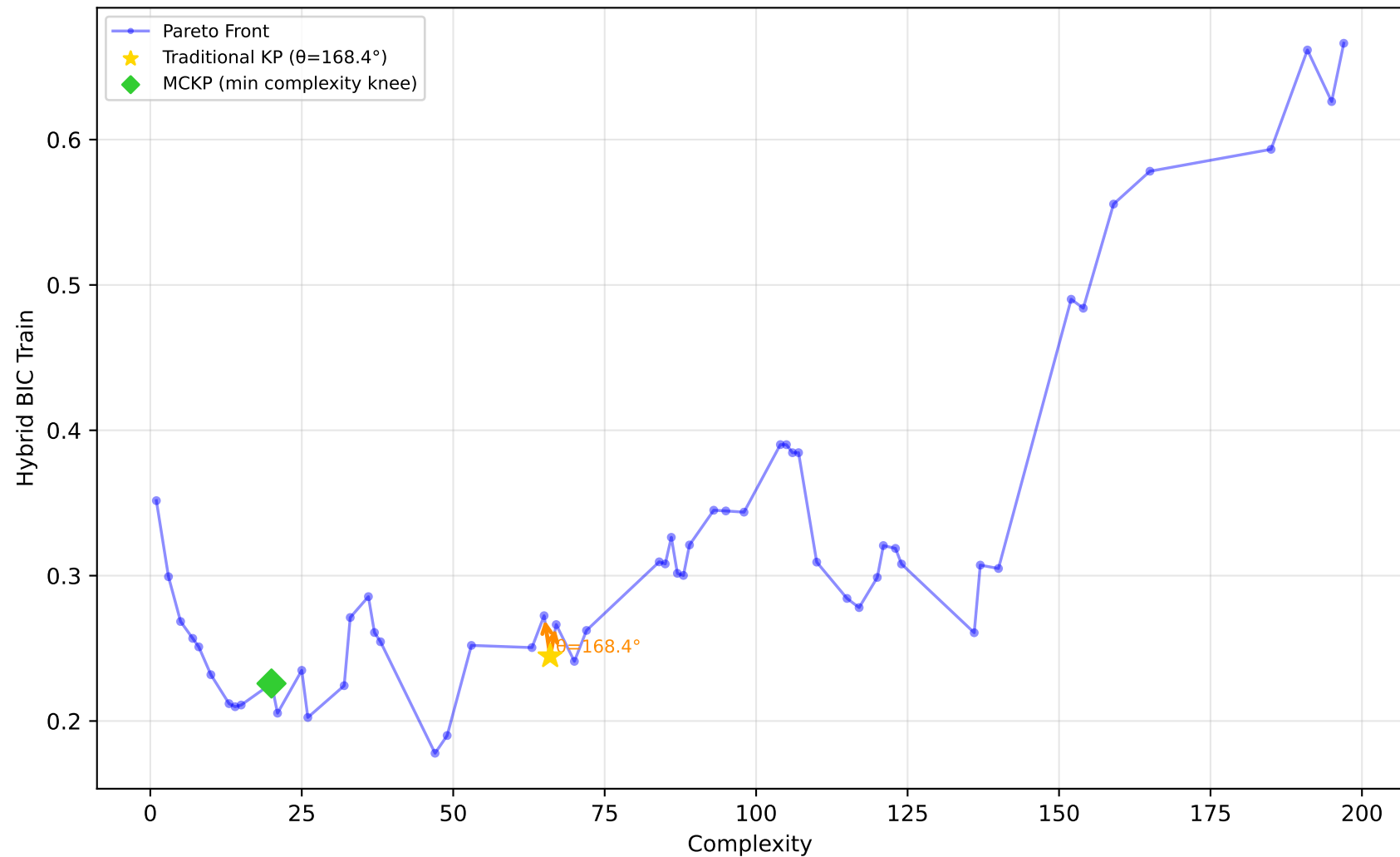
678_visualizing_environmental - Run 27 - SVP - Hybrid BIC Train \lambda_1=0.40, \lambda_2=0.00, \lambda_3=0.00 | Difficulty: 0.80 | Method: hmr
