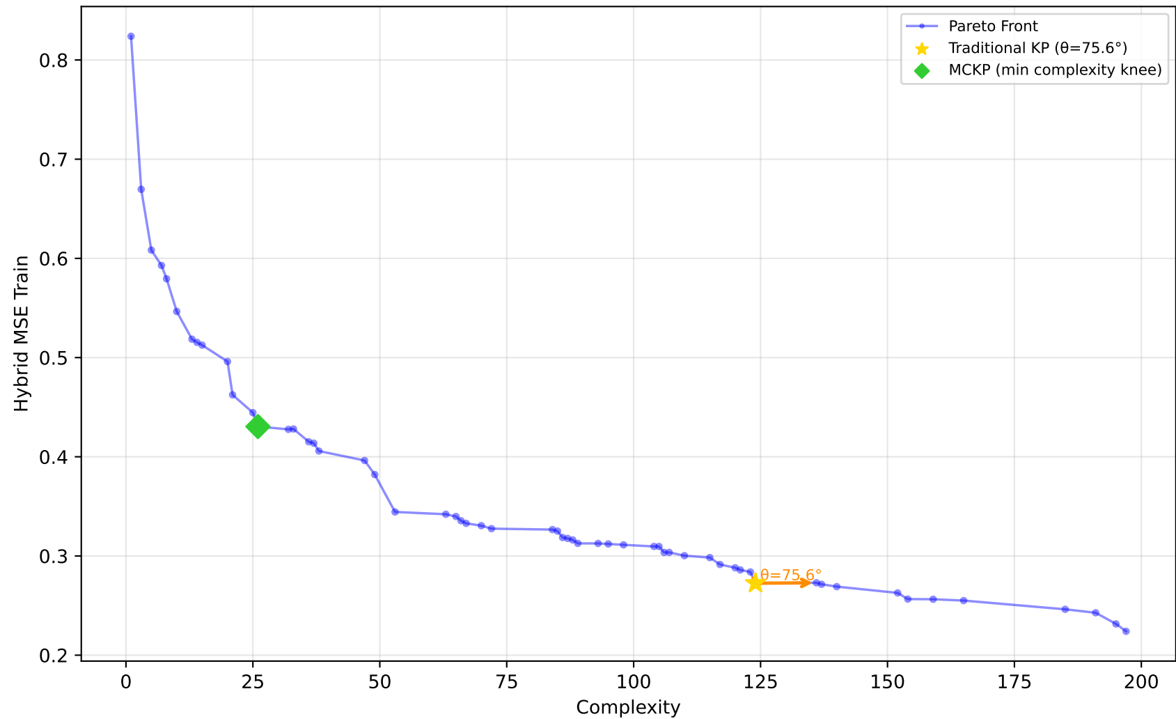
678_visualizing_environmental - Run 27 - SVP - Hybrid MSE Train \lambda_1=0.40, \lambda_2=0.00, \lambda_3=0.00 | Difficulty: 0.80 | Method: hmr
