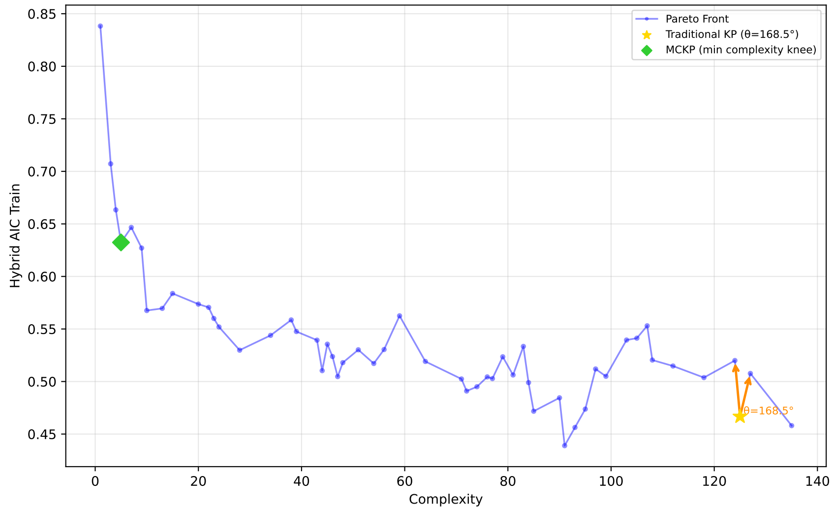
678_visualizing_environmental - Run 28 - MVP - Hybrid AIC Train \lambda_1=0.40, \lambda_2=0.00, \lambda_3=0.00 | Difficulty: 0.41 | Method: mckp
