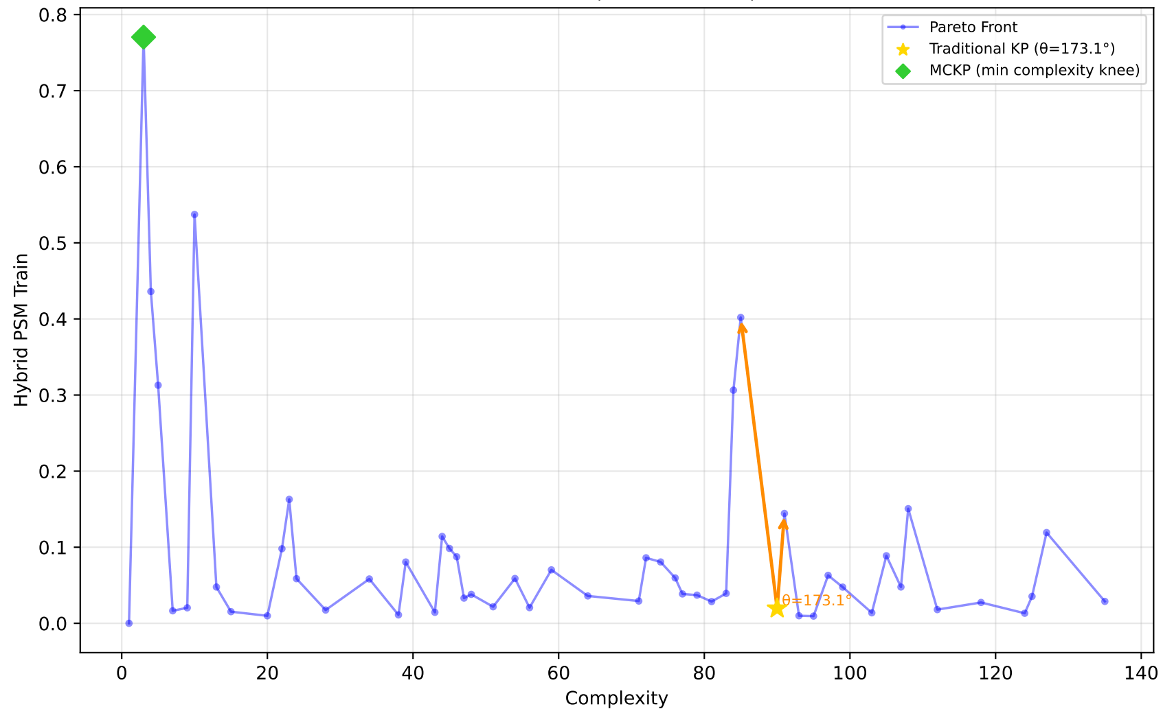
678_visualizing_environmental - Run 28 - MVP - Hybrid PSM Train \lambda_1=0.00, \lambda_2=0.00, \lambda_3=0.10 | Difficulty: 0.41 | Method: mckp
