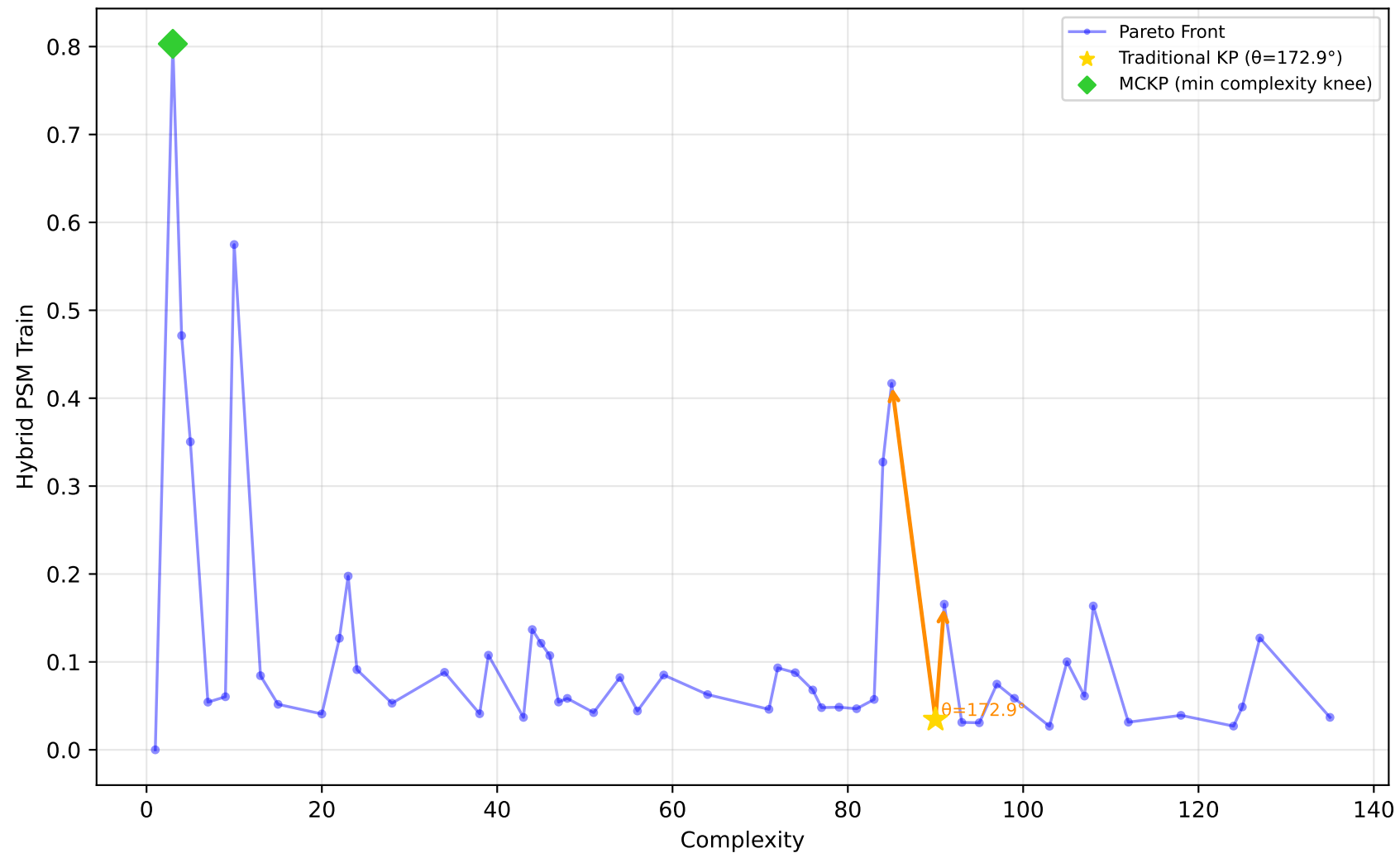
678_visualizing_environmental - Run 28 - MVP - Hybrid PSM Train \lambda_1=0.40, \lambda_2=0.00, \lambda_3=0.00 | Difficulty: 0.41 | Method: mckp
