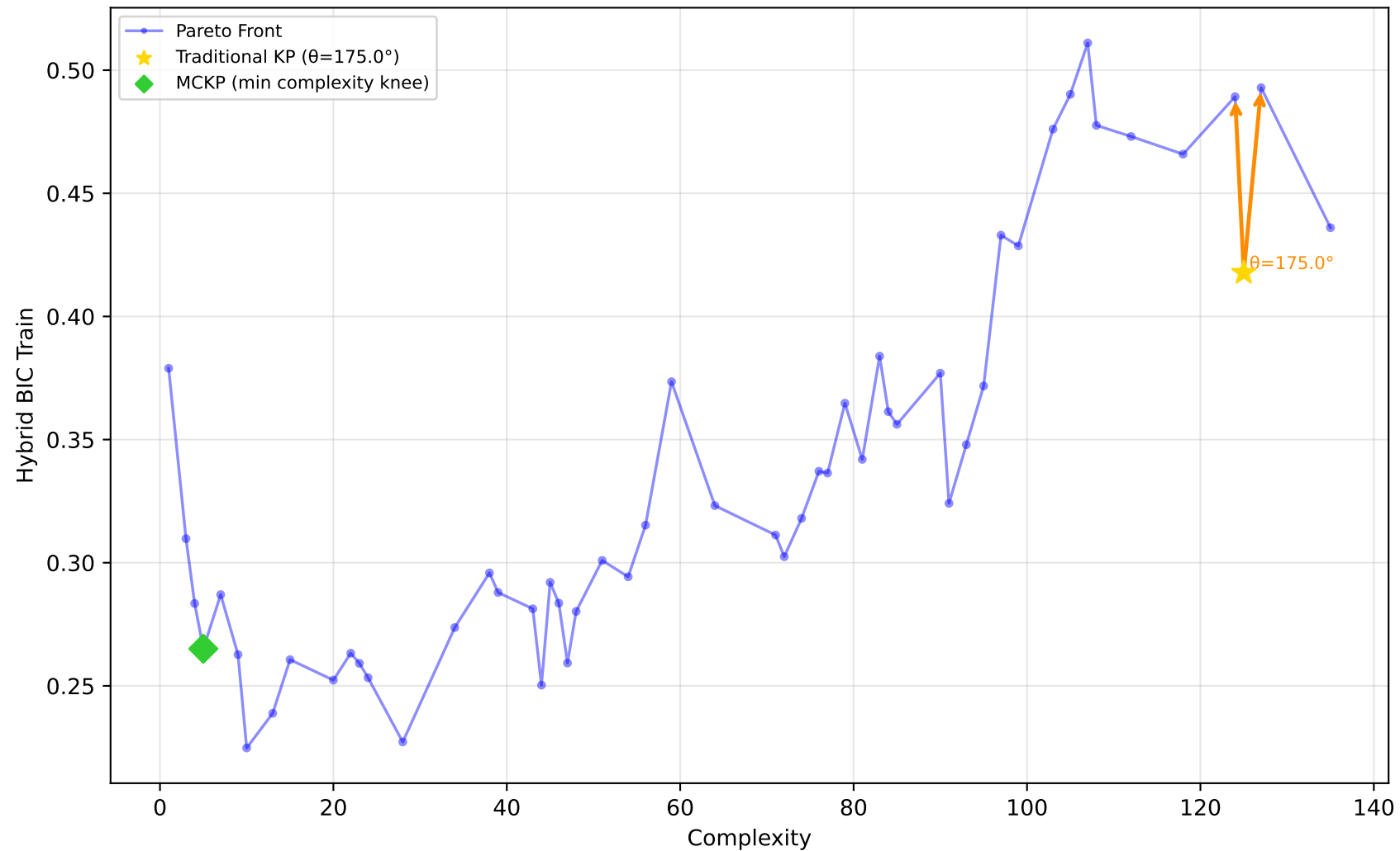
678_visualizing_environmental - Run 28 - SVP - Hybrid BIC Train \lambda_1=0.40, \lambda_2=0.00, \lambda_3=0.00 | Difficulty: 0.41 | Method: mckp
