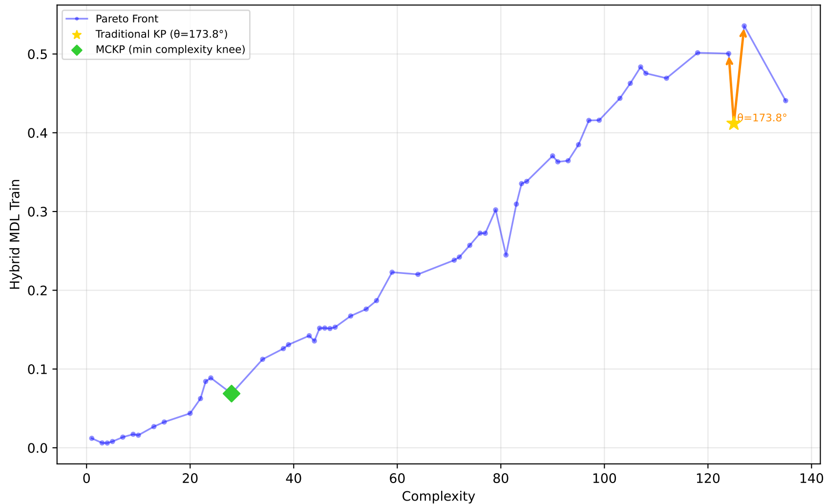
678_visualizing_environmental - Run 28 - SVP - Hybrid MDL Train \lambda_1=0.00, \lambda_2=0.10, \lambda_3=0.20 | Difficulty: 0.41 | Method: mckp
