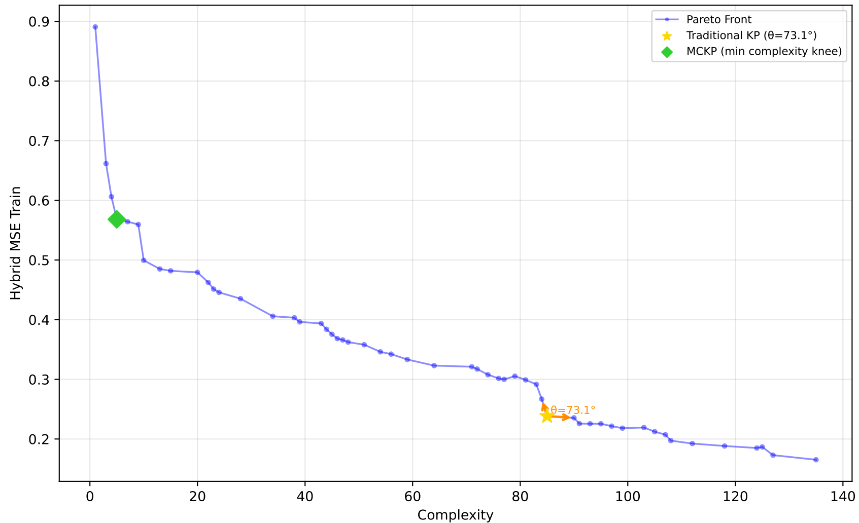
678_visualizing_environmental - Run 28 - SVP - Hybrid MSE Train \lambda_1=0.00 , \lambda_2=0.10 , \lambda_3=0.20 | Difficulty: 0.41 | Method: mckp
