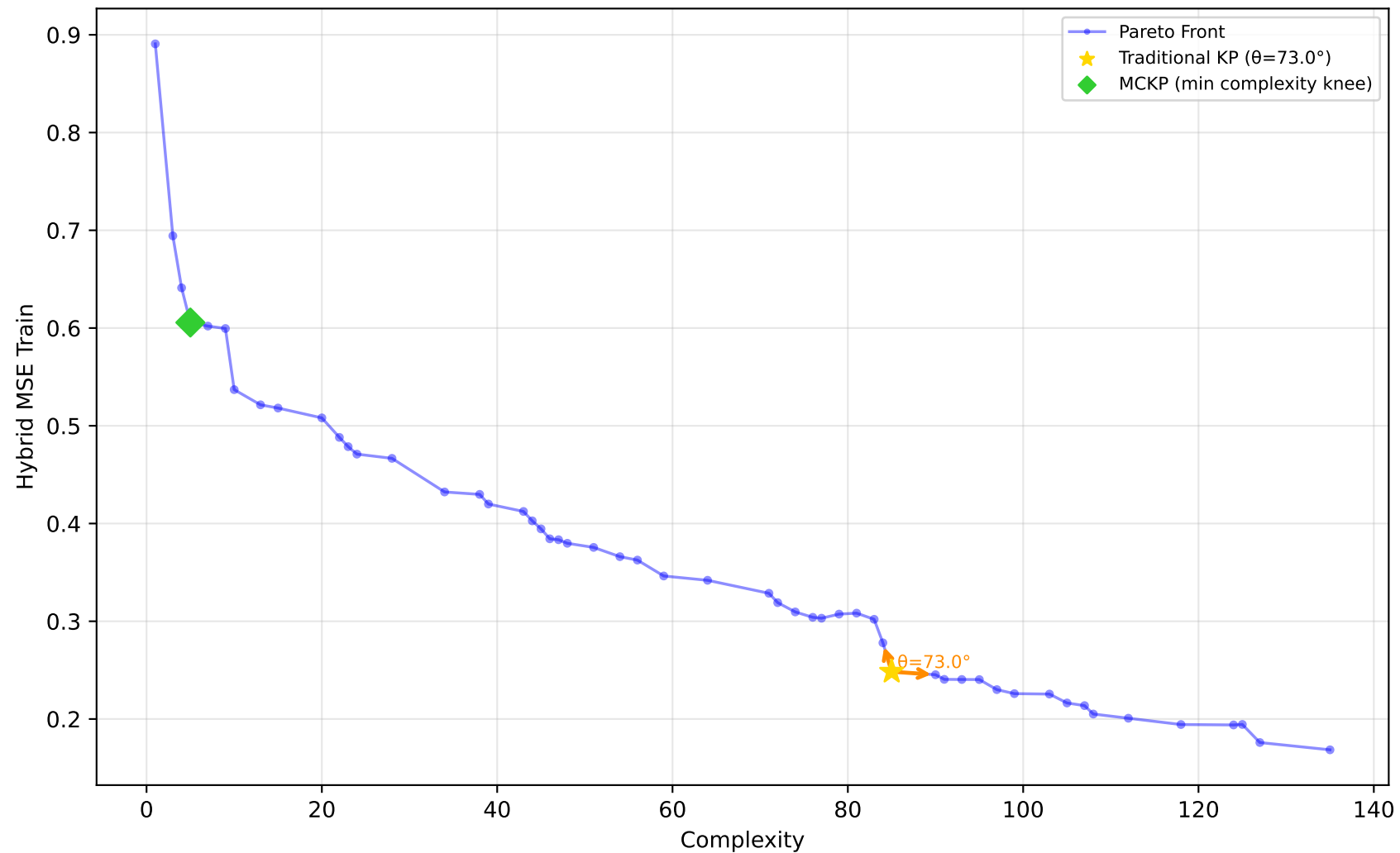
678_visualizing_environmental - Run 28 - SVP - Hybrid MSE Train \lambda_1=0.40, \lambda_2=0.00, \lambda_3=0.00 | Difficulty: 0.41 | Method: mckp
