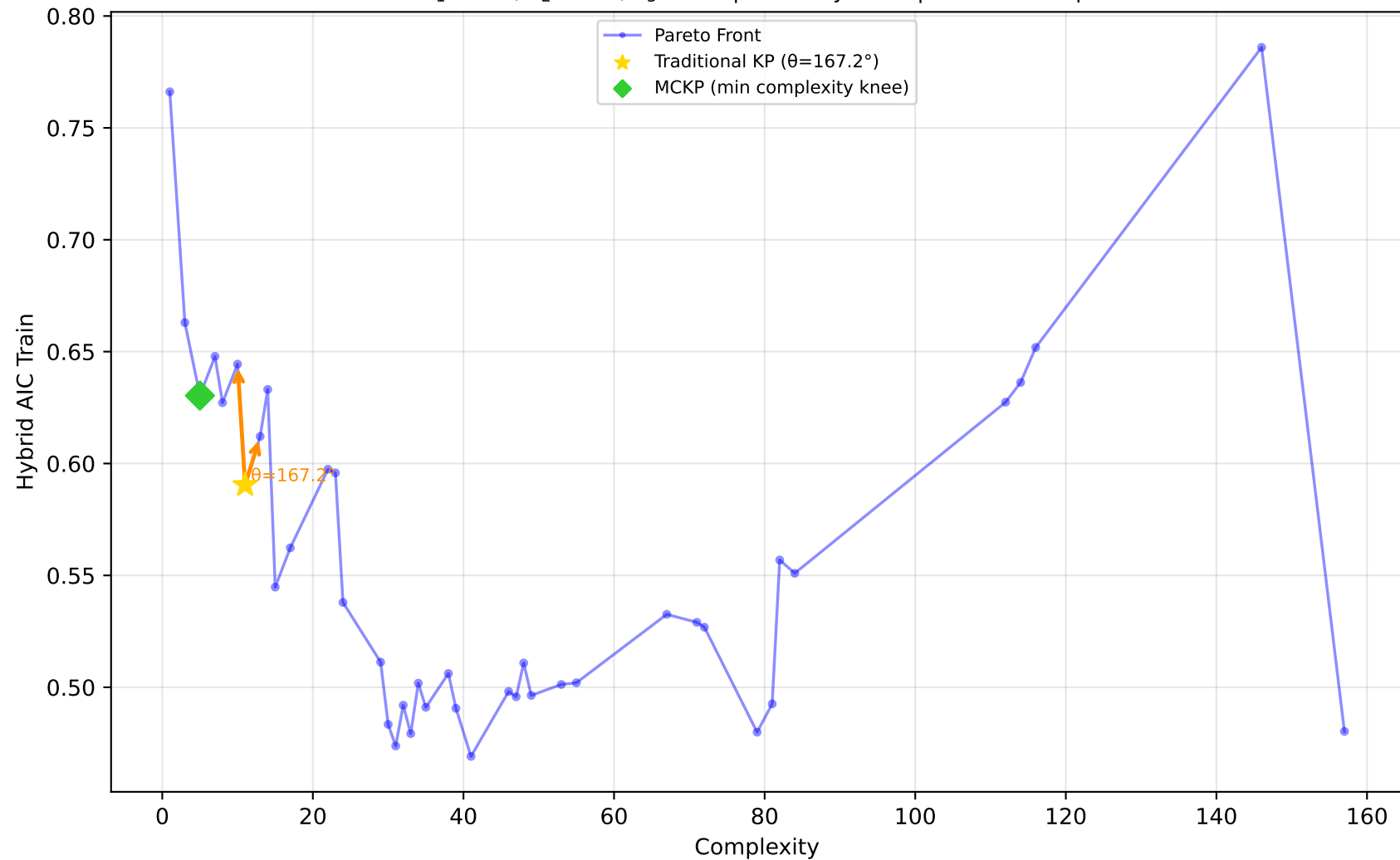
678_visualizing_environmental - Run 29 - MVP - Hybrid AIC Train \lambda_1=0.40 , \lambda_2=0.00 , \lambda_3=0.00 | Difficulty: 0.53 | Method: mckp
