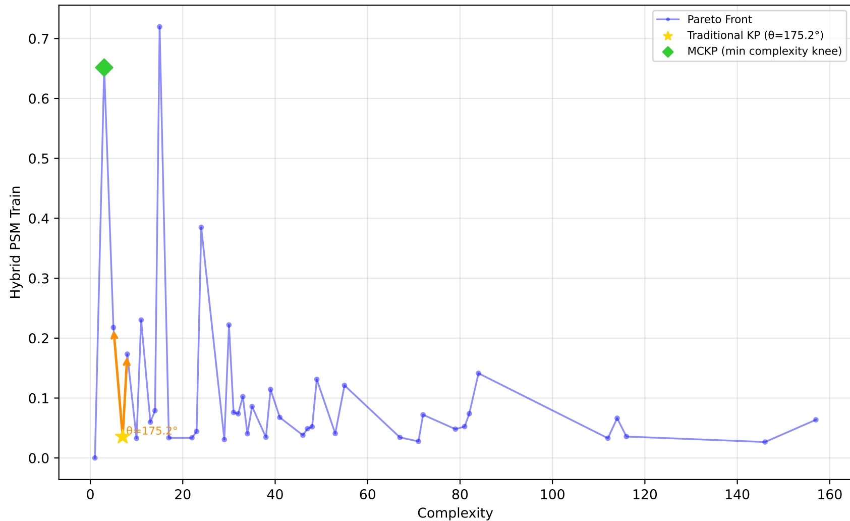
678_visualizing_environmental - Run 29 - MVP - Hybrid PSM Train \lambda_1=0.40 , \lambda_2=0.00 , \lambda_3=0.00 | Difficulty: 0.53 | Method: mckp
