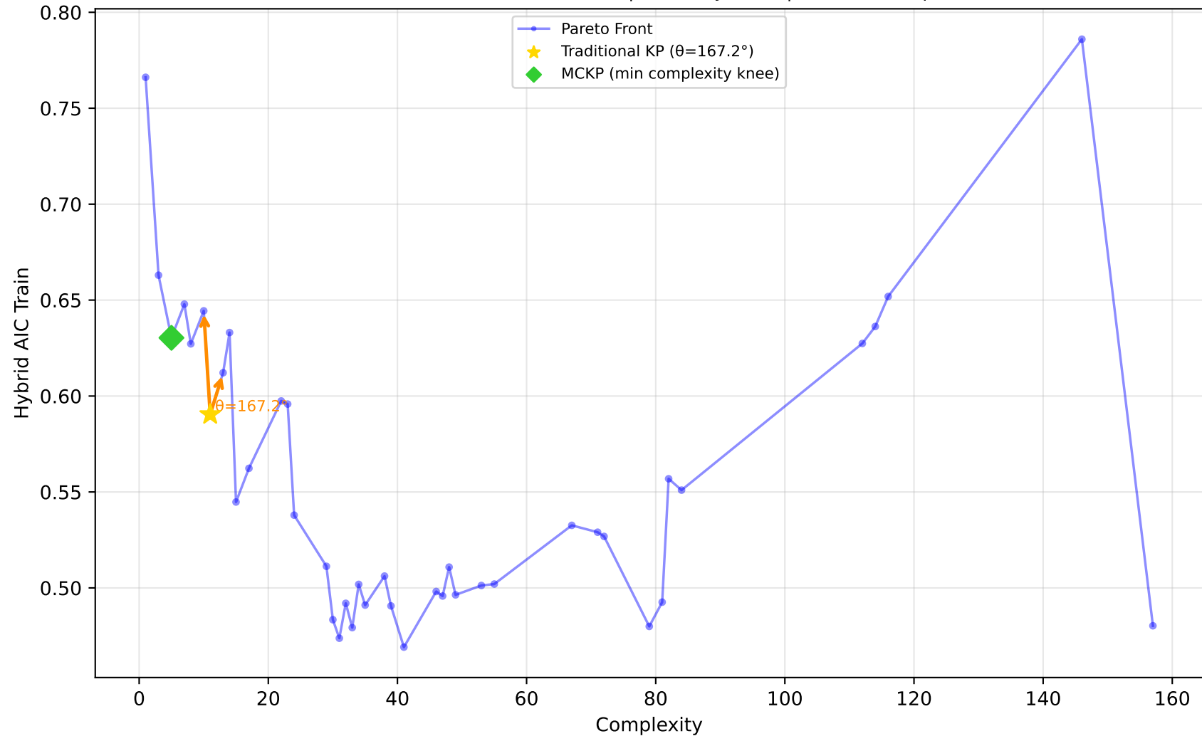
678_visualizing_environmental - Run 29 - SVP - Hybrid AIC Train \lambda_1=0.40 , \lambda_2=0.00 , \lambda_3=0.00 | Difficulty: 0.53 | Method: mckp
