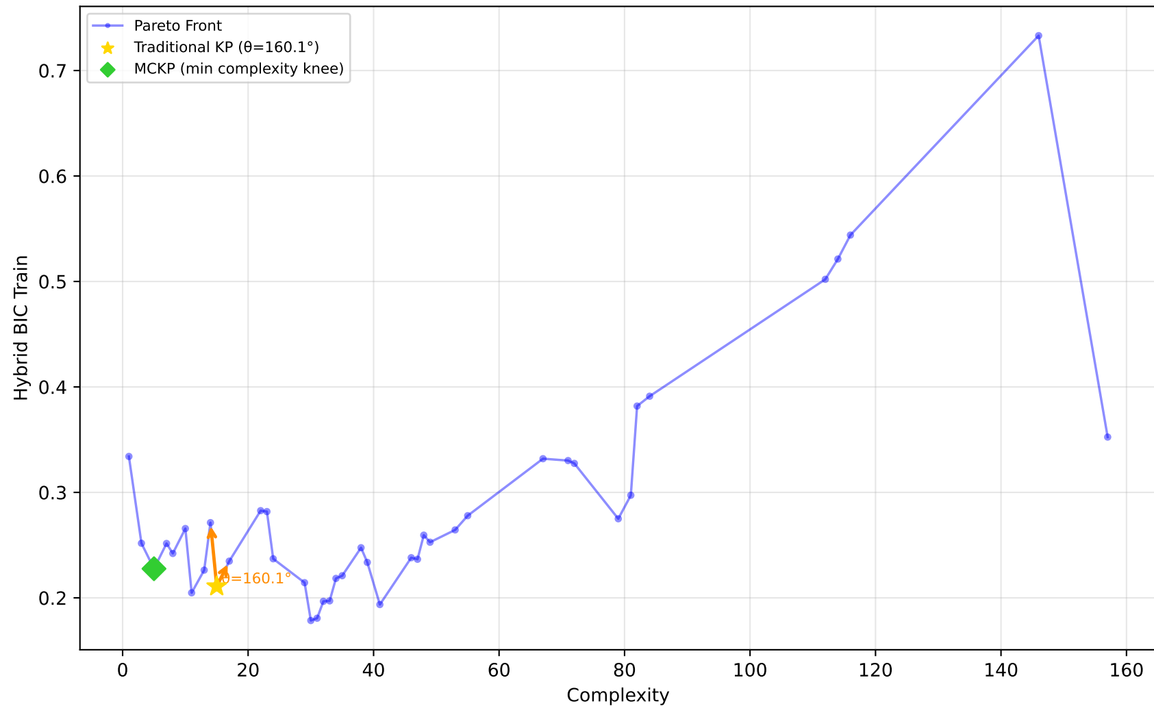
678_visualizing_environmental - Run 29 - SVP - Hybrid BIC Train \lambda_1=0.00, \lambda_2=0.10, \lambda_3=0.20 | Difficulty: 0.53 | Method: mckp
