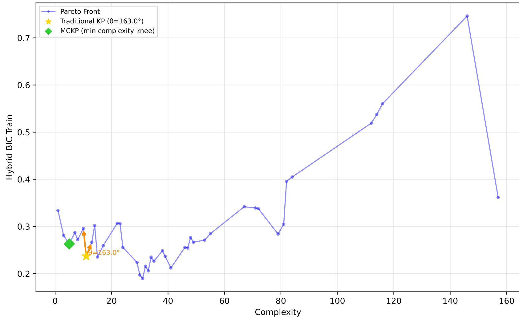
678_visualizing_environmental - Run 29 - SVP - Hybrid BIC Train \lambda_1=0.40, \lambda_2=0.00, \lambda_3=0.00 | Difficulty: 0.53 | Method: mckp
