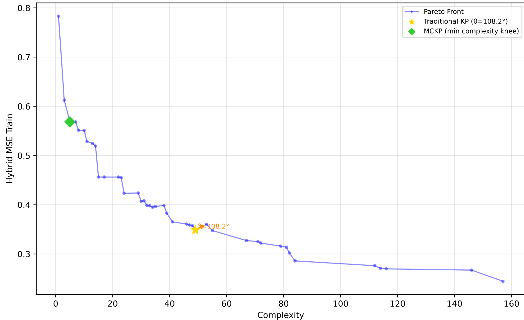
678_visualizing_environmental - Run 29 - SVP - Hybrid MSE Train \lambda_1=0.00, \lambda_2=0.10, \lambda_3=0.20 | Difficulty: 0.53 | Method: mckp
