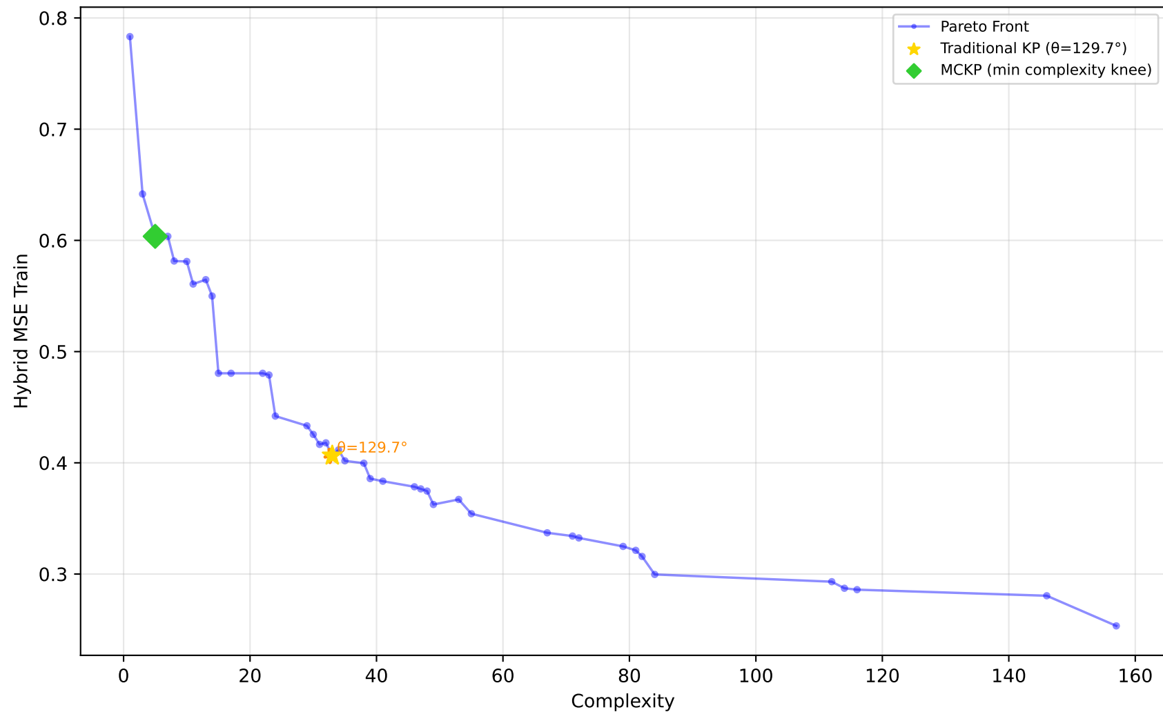
678_visualizing_environmental - Run 29 - SVP - Hybrid MSE Train \lambda_1=0.40 , \lambda_2=0.00 , \lambda_3=0.00 | Difficulty: 0.53 | Method: mckp
